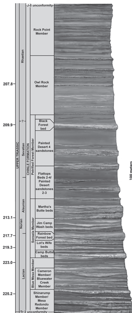
Stratigraphic section of the Chinle Formation in Northern Arizona
