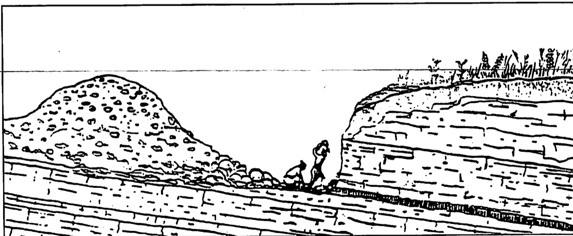
Pencil sketch showing geologic cross section of quarry, pipestone is the dark stratum near the bottom of the quarry.
