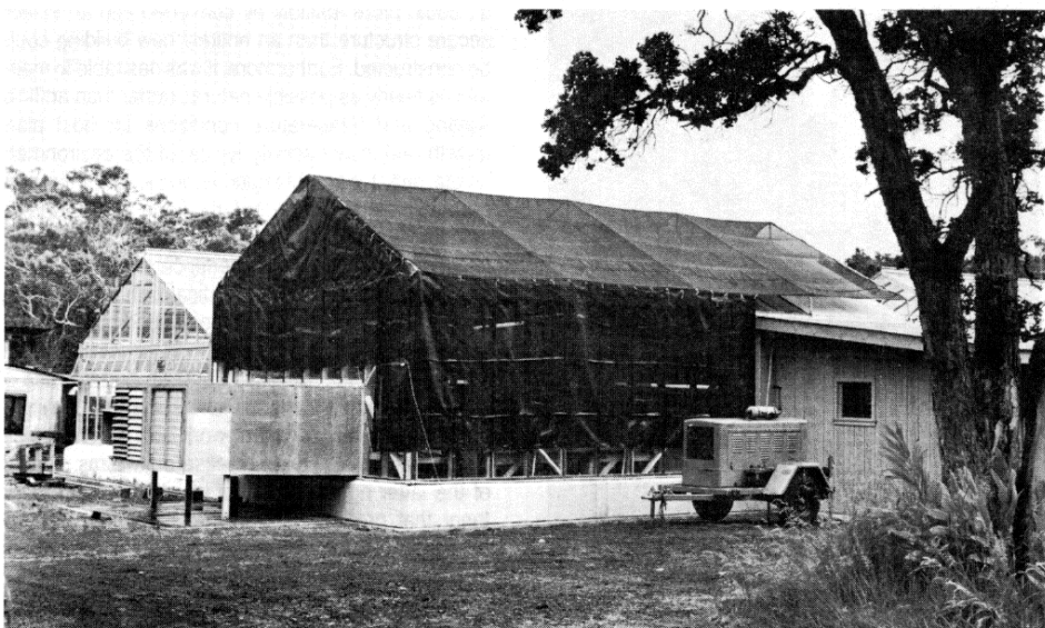
NPS quarantine facility at Hawaii Volcanoes National Park is designed as a greenhouse with natural sunlight and cooled by moving outside air through the secure area with large fans. The picture shade cloth is used in the summer to help control the inside temperature.
