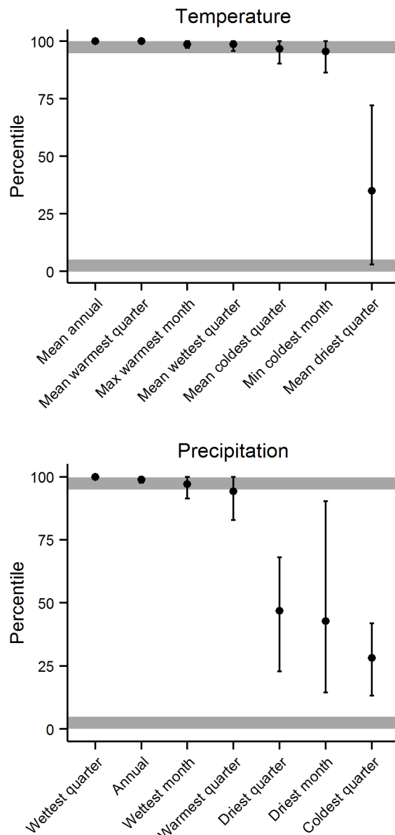
Figure 2. Recent temperature and precipitation percentiles at Acadia National Park (including areas within 30-km [18.6-mi] of the park’s boundary). Black dots indicate average recent percentiles across the 10, 20, and 30-year intervals (moving windows). Variables are considered “extreme” if the mean percentiles are <5 th percentile or >95 th percentile (i.e., the gray zones, where recent climate is pushing the limits of all observed climates since the year 1901). Black bars indicate the range of recent percentiles across 10, 20, and 30-year moving windows (larger bars indicate higher sensitivity to moving window size).
