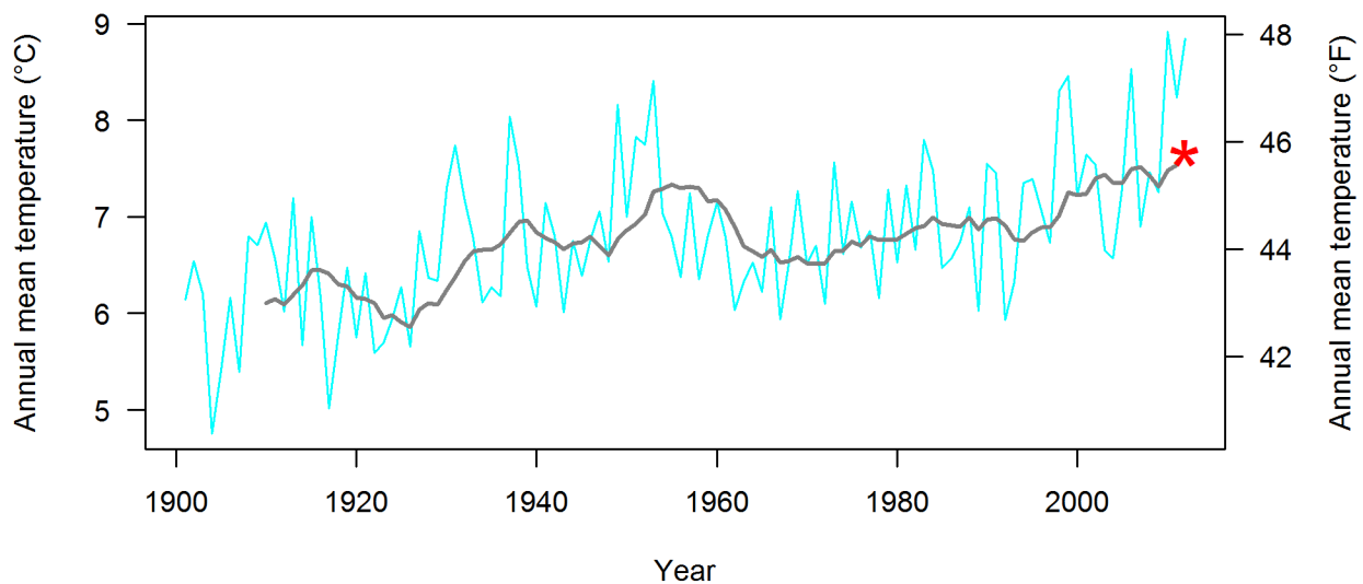
Figure 1. Time series used to characterize the historical range of variability and most recent percentile for annual mean temperature at Acadia National Park (including areas within 30-km [18.6-mi] of the park’s boundary). The blue line shows temperature for each year, the gray line shows temperature averaged over progressive 10-year intervals (10-year moving windows), and the red asterisk shows the average temperature of the most recent 10-year moving window (2003–2012). The most recent percentile is calculated as the percentage of values on the gray line that fall below the red asterisk (see results of most recent percentiles for all temperature and precipitation variables in Figure 2).
