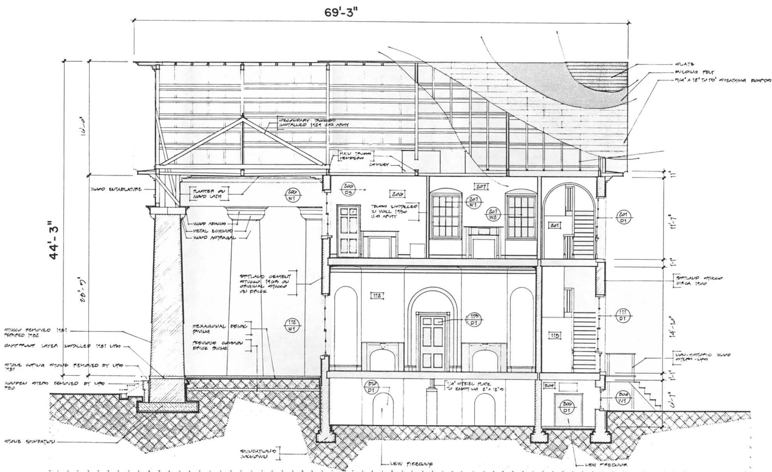
1 8 TRANSVERSE SECTION - MAIN BLOCK SCALE - 1/4" = 1'-0"
