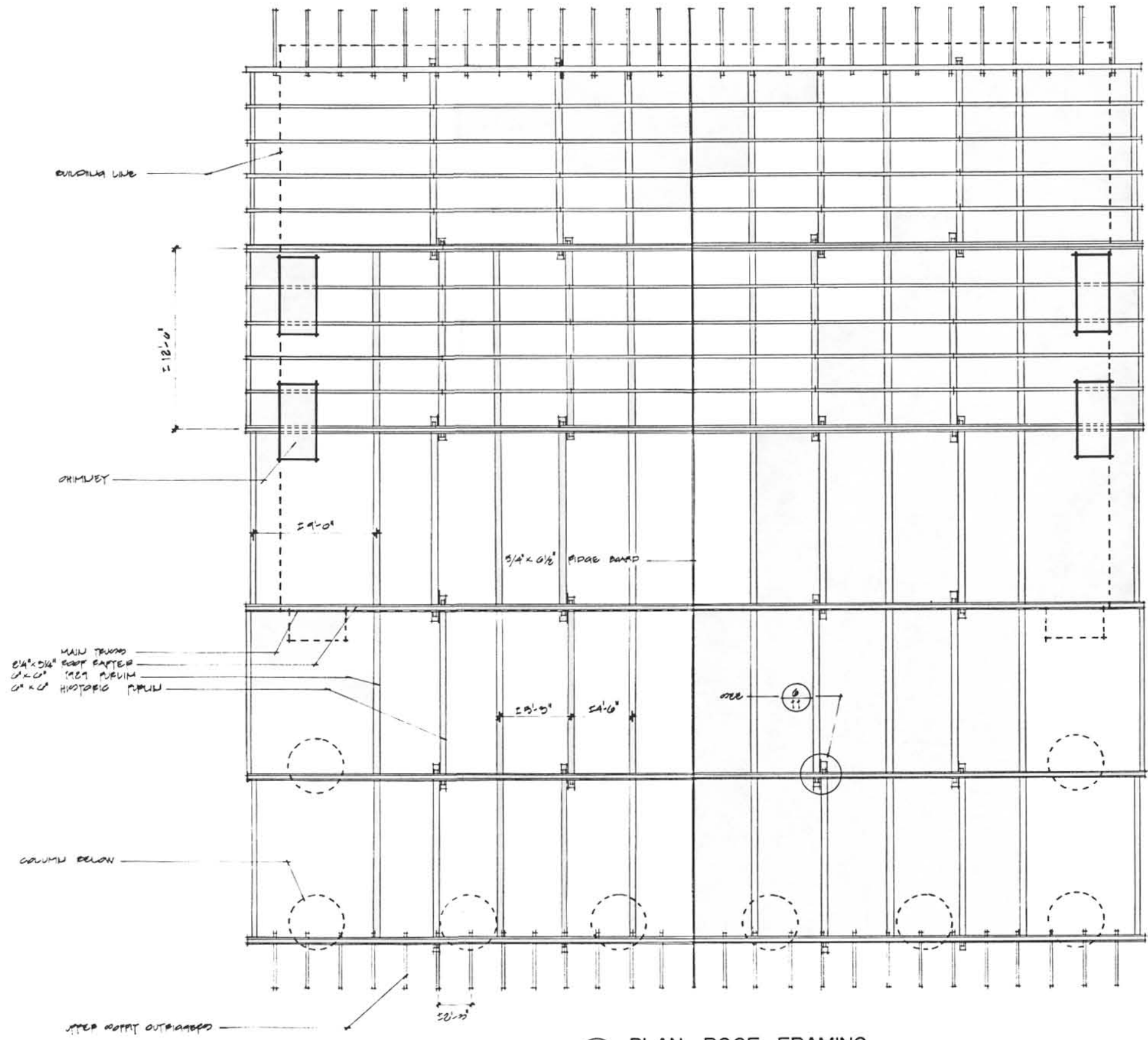
1 10 PLAN · ROOF FRAMING SCALE: 1/4" = 1'-0"
