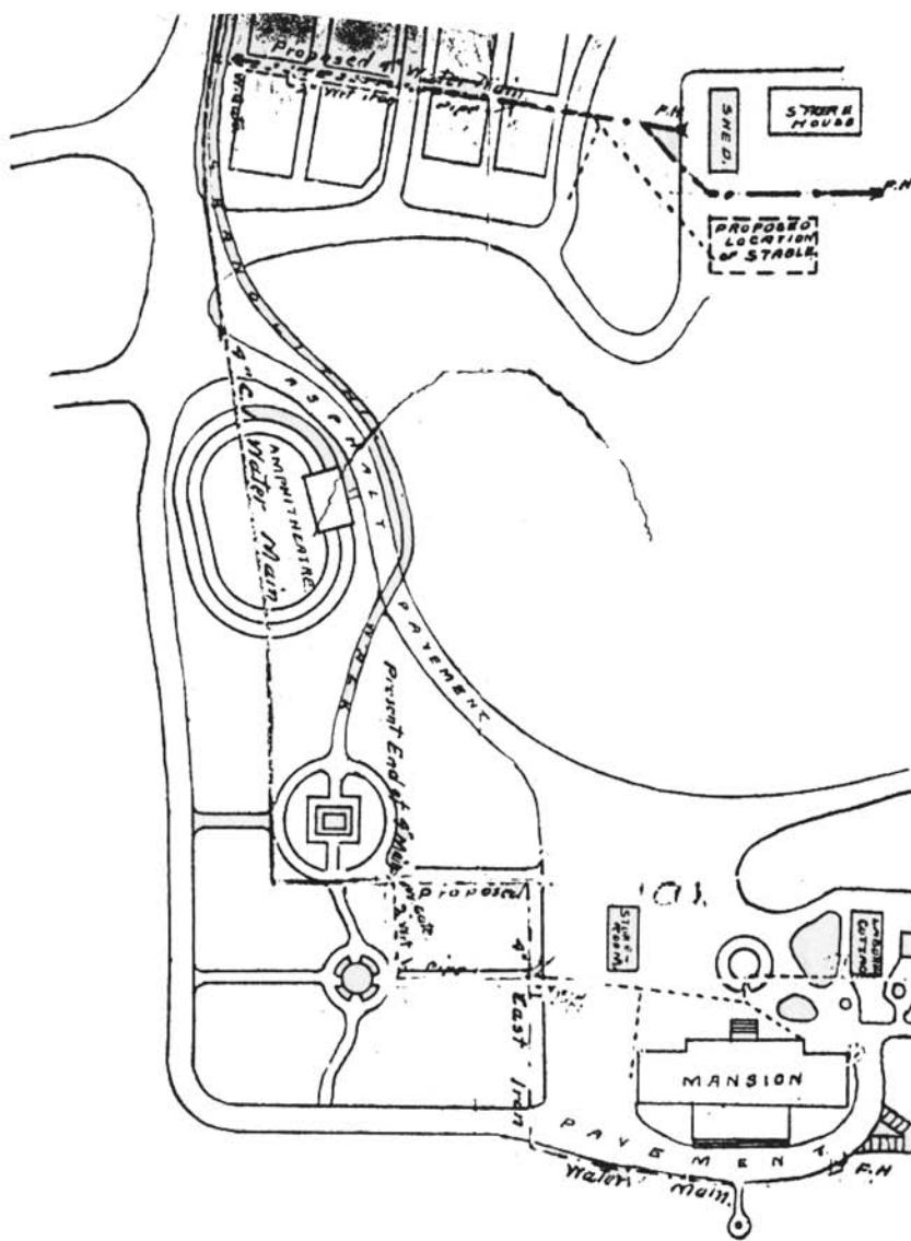
MAP SHOWING PROPOSED EXTENSION OF WATER MAIN AND LOCATION OF FIRE HYDRANTS AT ARLINGTON WAT. CEMETERY.
