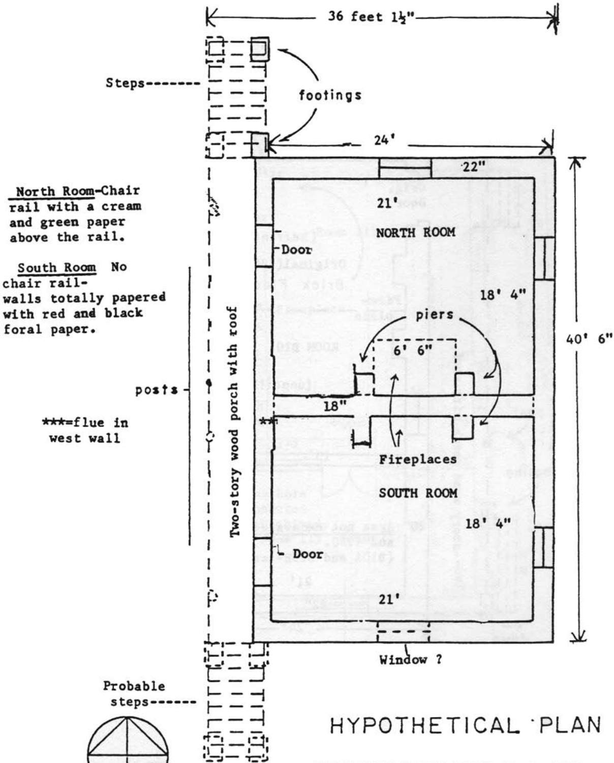
NORTH WING SECOND FLOOR PLAN, 1802
