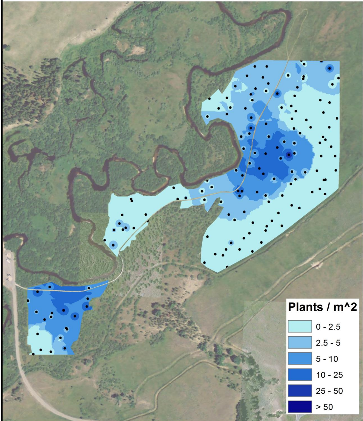
Figure 1. The sampling frame along the Big Hole River floodplain in BIHO, with 2012 quadrat locations (black points) and predicted patterns of camas density based on a kriging interpolation from 2012 established camas plant counts.
