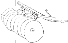
Eight-disc horse-drawn plow-bottom disk plow
