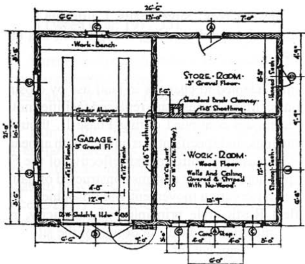
- FLOOR PLAN - . Scale \frac{1}{4}'' = 1'-0'' .
