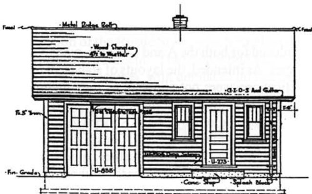
- FRONT - ELEVATION - . Scale \frac{1}{4}'' = 1'-0'' .
