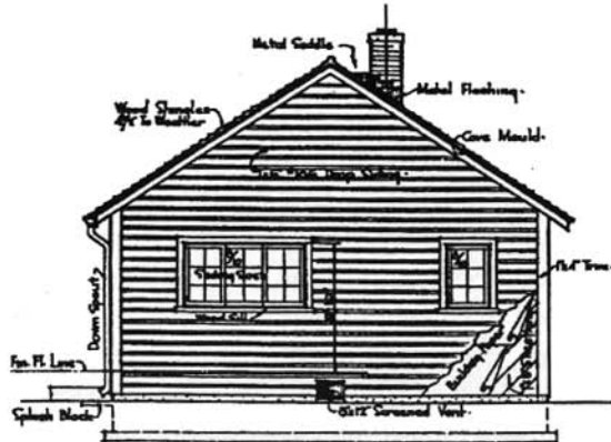
- SIDE - ELEVATION - . Scale \frac{1}{4}'' = 1'-0'' .
