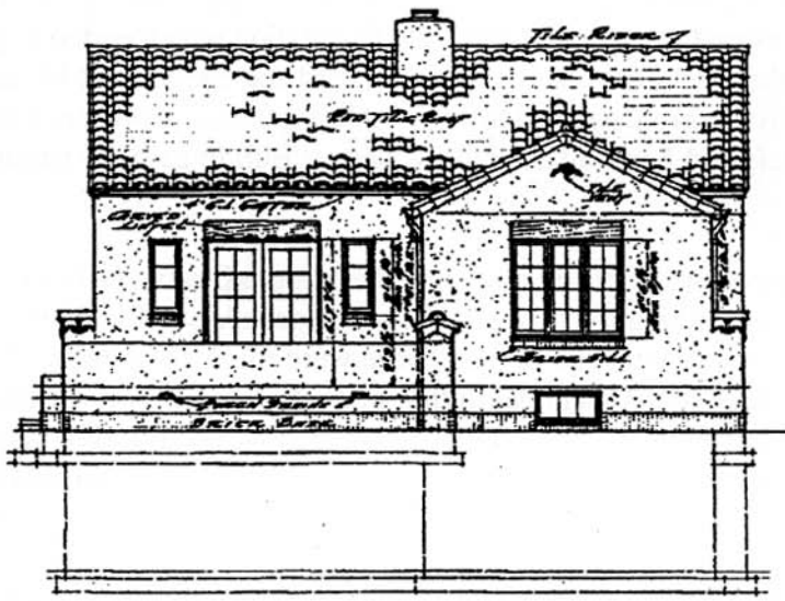
SOUTH ELEVATION
