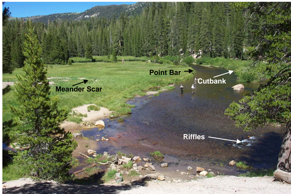
Figure 15. The Middle Fork of the San Joaquin River meanders through Soda Springs Meadow, creating geomorphic features such as point bars, cut banks, and in-stream riffles. A meander scar defines the pattern of a previous channel. Modified from a National Park Service photograph, available at: http://www.nps.gov/depo/photosmultimedia/photogallery.htm . Accessed November 2009.
