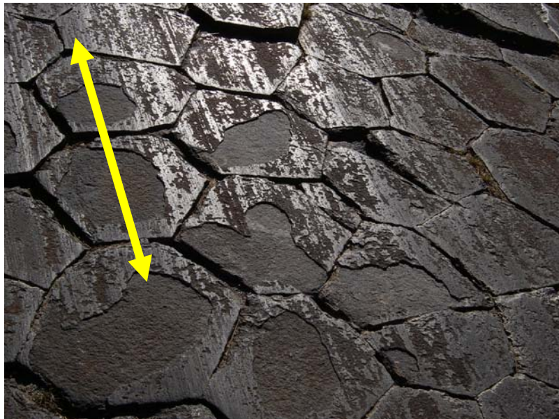
Figure 7. Glacial polish and glacial striations (parallel scratches or lines) on the top of the columns at Devils Postpile National Monument. Glacial abrasion caused both features. Due to weathering or illegal collecting, some of the glacial polish has been removed from the polygonal tops of the Postpile. Striations provide directional evidence, as well. In this picture, the last glacier followed one of two directions, as indicated by the yellow arrow. Modified from a National Park Service photograph by David Scott, available at: http://www.nps.gov/depo/photosmultimedia/photogallery.htm . Accessed November 2009.
