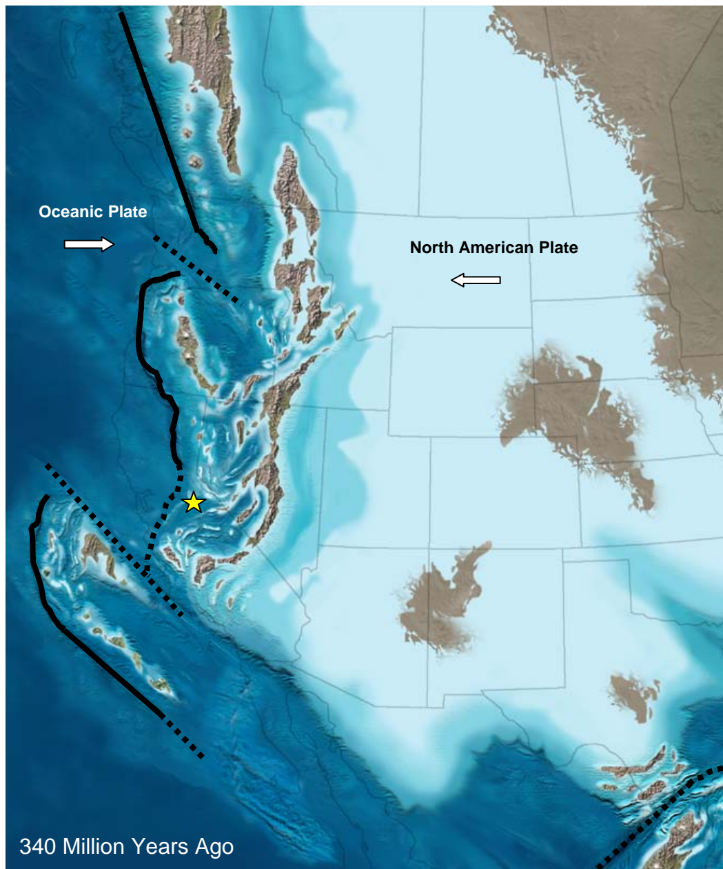
Figure 19. Early Mississippian paleogeographic map of southwestern North America. Approximately 340 million years ago, the western margin of North America was an “active” tectonic margin with a slab of oceanic lithosphere being subducted beneath the North American continent. The Antler Orogeny (mountain-building episode) caused mountains to emerge in central Nevada and Idaho and a major transgression to spread marine environments across western North America. The black line (dashed where uncertain) represents the general location of subduction zones and active margins that bordered western and southeastern North America in the Devonian and Mississippian. The yellow star represents the approximate location of today’s Devils Postpile National Monument. The brown color denotes land, light blue represents shallow marine, and dark blue represents deeper marine environments. The general direction of movement of both plates is indicated by the white arrows. Modified from Dr. Ron Blakey (Northern Arizona University), available online at: http://jan.ucc.nau.edu/rcb7/garm340.jpg . Accessed November 2009.
