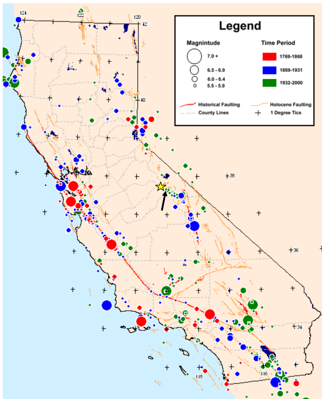
Figure 5. Historical earthquake map of California. The yellow star (not to scale) represents the approximate location of Devils Postpile National Monument. The arrow points to the location of the 1980 earthquakes near Mammoth Lakes, California. Modified from California Geological Survey graphic, available at: http://redirect.conservation.ca.gov/cgs/rghm/quakes/historical/index.htm . Accessed November 2009.
