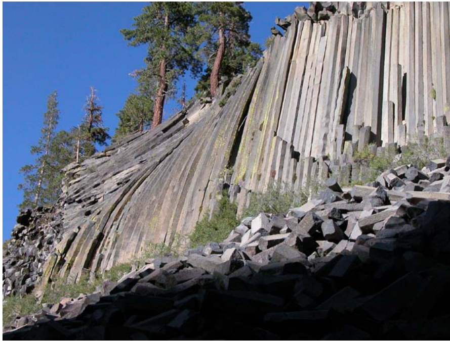
Figure 3. Basalt columns of the Devils Postpile. Uniform composition and thickness resulted in exceptionally long, vertical columns (about 20 m or 60 ft long). Differences in composition, thickness, cooling rates, and other irregularities produced the curved columns to the left of the vertical columns. Column collapse has created a talus pile at the base of the columns. National Park Service photograph, available at: http://www.nps.gov/depo/photosmultimedia/photogallery.htm . Accessed November 2009.
