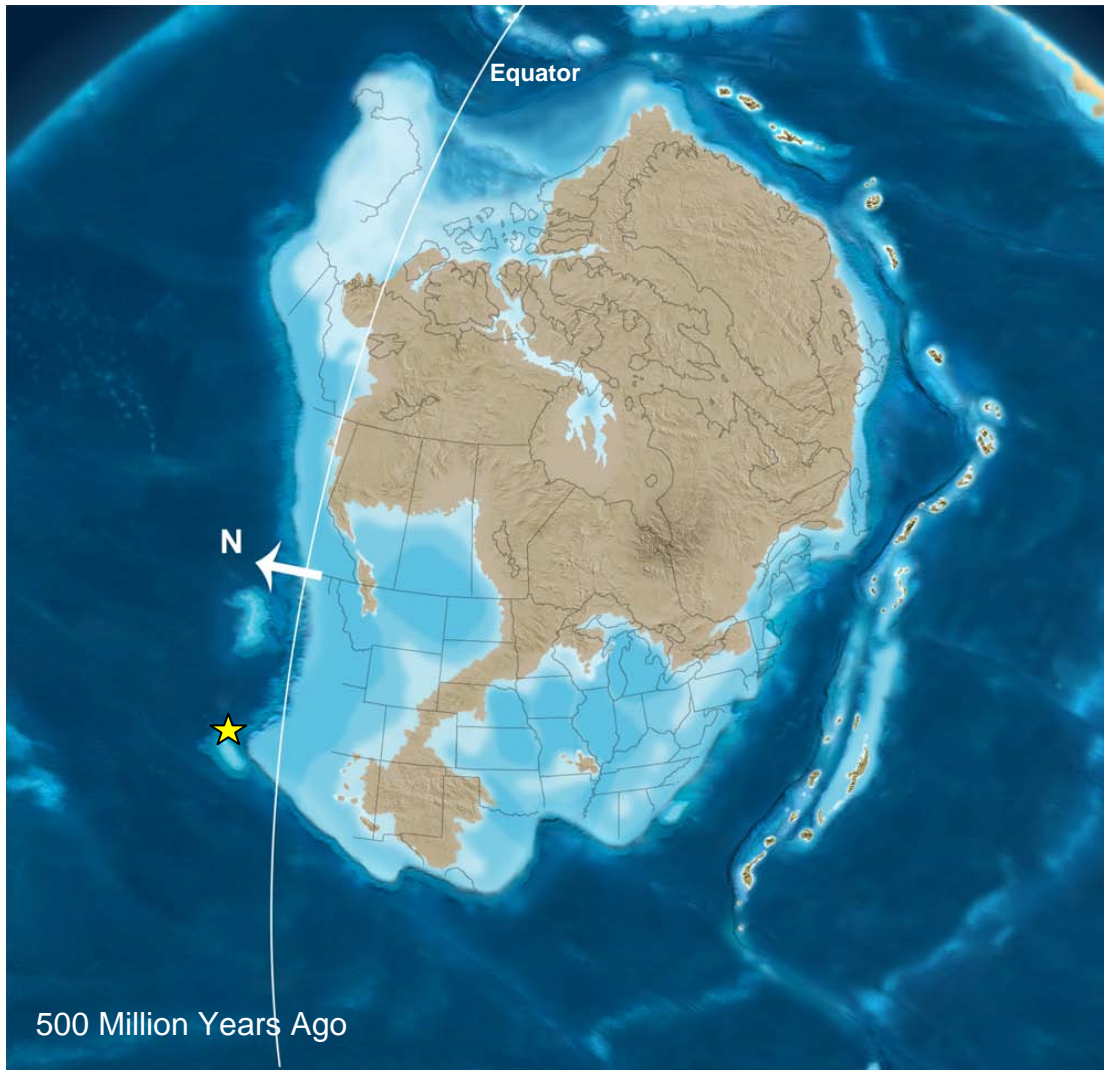
Figure 18. Late Cambrian paleogeographic map of North America. Approximately 500 million years ago, the Sierra Nevada region and future site of Devils Postpile National Monument (yellow star) lay offshore of the “passive” western margin of the emerging North America continent. The brown color indicates exposed land, light blue represents shallow marine, and dark blue shows deep marine. Map modified from the Late Cambrian map of Dr. Ron Blakey (Northern Arizona University), available online at: http://jan.ucc.nau.edu/rcb7/namC500.jpg . Accessed November 2009.
