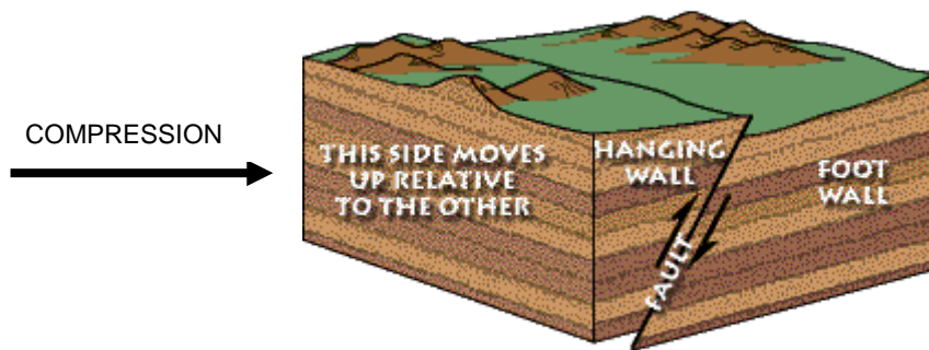
B) Reverse (thrust) Fault
