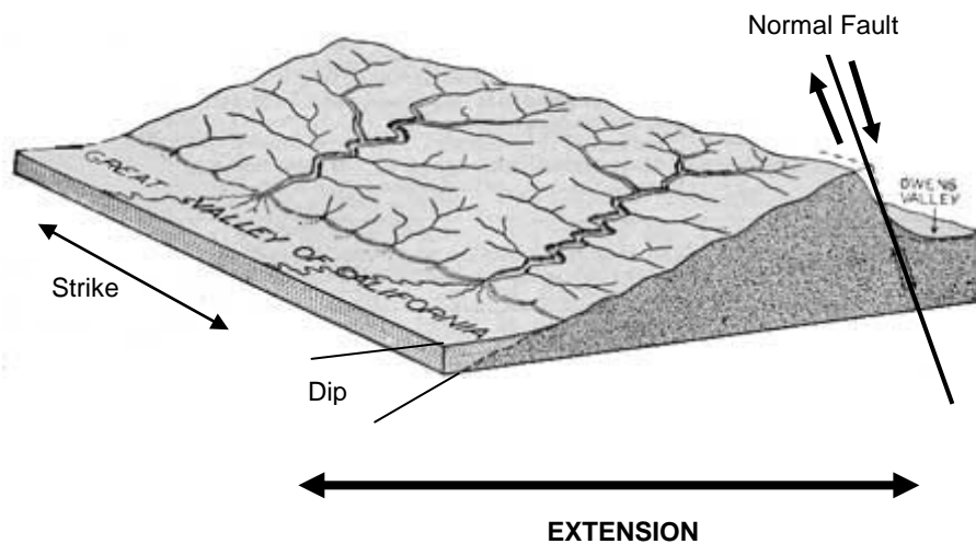
Figure 2. The Sierra Nevada fault block. The historic view of the Sierra Nevada shows the great eastern escarpment that rises nearly 3 km (2 mi) from Owens Valley (foreground). The generalized diagram illustrates the origin of the Sierra Nevada fault block. As tectonic forces pulled apart the region (Basin- and- Range extension), the Sierra Nevada was tilted upwards (relative to the Owens Valley block) along a basin-bounding normal fault. The “dip” of the beds is the angle the beds make with the surface, while the “strike” represents the compass direction that the inclined beds make when they intersect the surface. For an explanation of the various types of faults, see figure 17. Both the photograph and diagram are from Matthes (1930). The photograph is also available online from the U.S. Geological Survey photographic library at: http://libraryphoto.cr.usgs.gov/html/lib/btch432/btch432j/btch432z/mwc01116.jpg . The diagram is available online at: http://www.nps.gov/history/history/online_books/geology/publications/pp/160/sec2a.htm . Both accessed November 2009.
