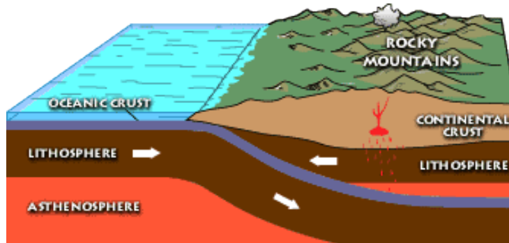
B) "Flat slab"-style subduction that gave rise to the Laramide Orogeny and the Rocky Mountains.
