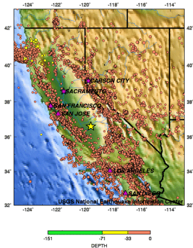
Figure 6. Seismicity of California showing earthquakes from 1990 to 2006. The colored circles designate earthquake locations, with the various colors indicating depth ranges in kilometers (see depth key above). Note that most of the earthquakes have occurred within 33 km (21 mi) of the surface. Purple triangles depict cities and purple stars depict state capitols. The yellow star (not to scale) represents the approximate location of Devils Postpile National Monument. Modified from U.S. Geological Survey graphic , available at: http://earthquake.usgs.gov/regional/states/california/seismicity.php . Accessed November 2009.
