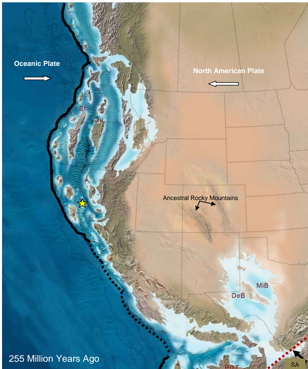
Figure 20. Late Permian paleogeographic map of southwestern North America. About 255 million years ago, the Sonoma Orogeny accreted marine sediments to the western margin of North America. South America (SA) continued to close the proto-Gulf of Mexico and collide with North America. Forces associated with this collision formed the northwest-southeast trending Ancestral Rocky Mountains. By the Late Permian, many of the basins that began forming in the Late Mississippian and Pennsylvanian had filled with sediment, but the Delaware Basin (DeB) and Midland Basin (MiB), prolific oil- and gas- producing basins, continued to subside. By the Triassic, all of the major landmasses had come together to form the supercontinent, Pangaea. The yellow star represents the approximate location of today's Devils Postpile National Monument. The black line marks the general trend of the subduction zone between the North American lithospheric plate and the oceanic plate. The dashed red line represents a very approximate location between South America and North America. The brown and yellowish-brown colors denote land, light blue represents shallow marine, and dark blue represents deeper marine environments. Modified from Dr. Ron Blakey (Northern Arizona University), available online at: http://jan.ucc.nau.edu/rcb77/garm255.jpg . Accessed November 2009.
