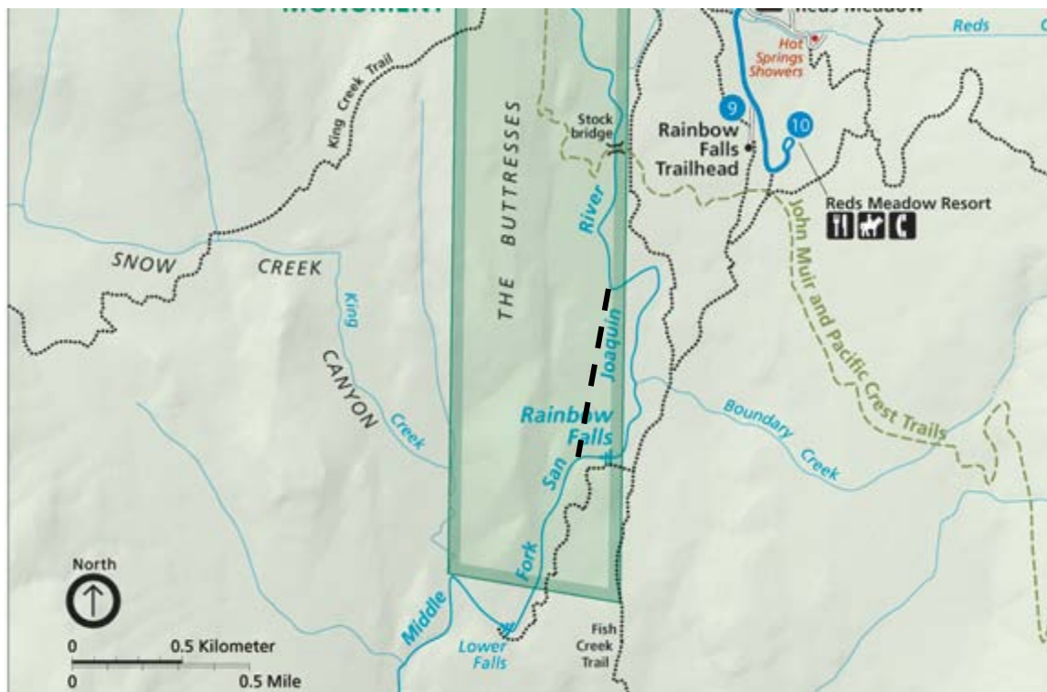
Figure 13. Original channel of the Middle Fork of the San Joaquin River, Devils Postpile National Monument. The dashed, black line depicts the original channel that eroded vertically through solidified lava flows. When the Middle Fork flowed back to its original channel from the east, it flowed over the previously eroded cliff of rhyodacite, forming Rainbow Falls. Modified from National Park Service map.
