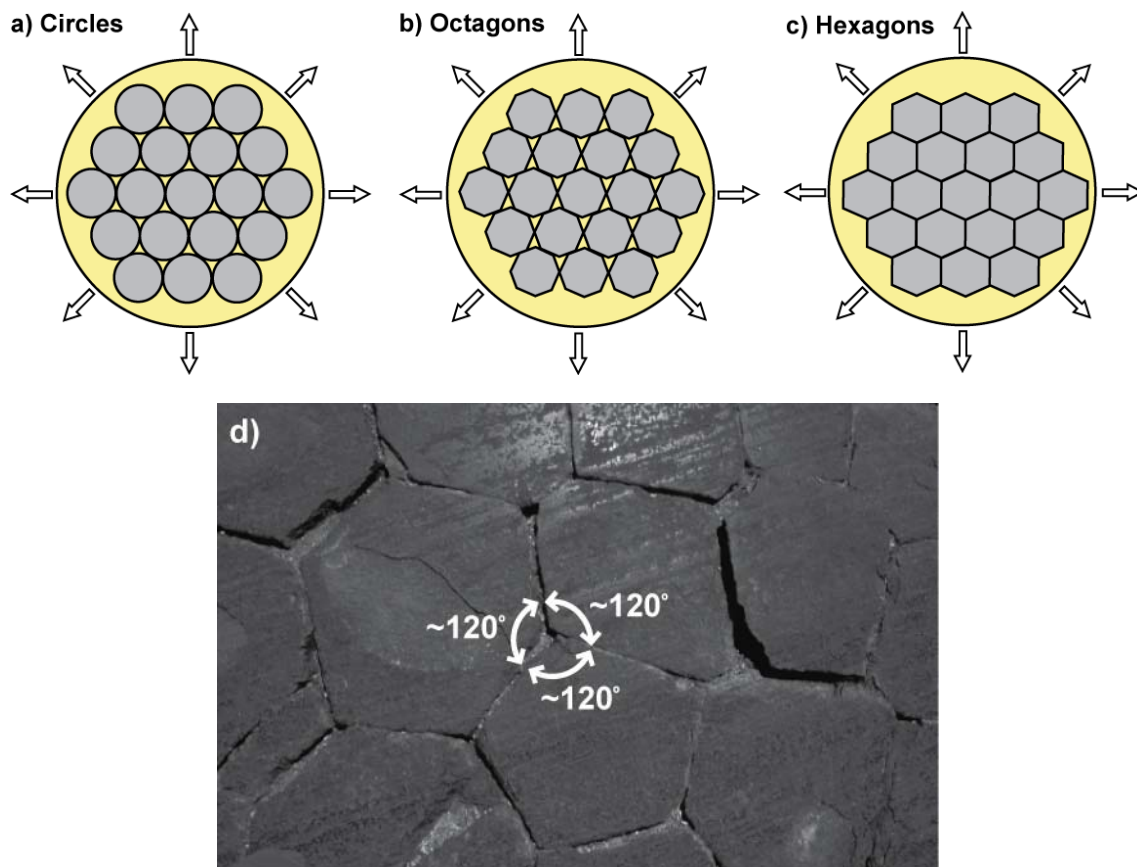
Figure 10. A hexagonal pattern is the ideal shape for columnar joints in basalt. If homogenous lava cools uniformly, it shrinks and is subject to tensional forces (white arrows) that are equal in all directions. Compared to circles (a) and octagons (b), the hexagon (c) fits most efficiently without gaps. The columnar joints at Devils Postpile NM have a large proportion of hexagonal columns, which is rare. Not all columns are hexagonal because lava is not completely homogenous and does not cool perfectly uniformly. As shown in (d), some columns are also 5-sided with joints intersecting at nearly 120-degree angles. Graphics and photograph modified from Lillie (2005), used with permission.
