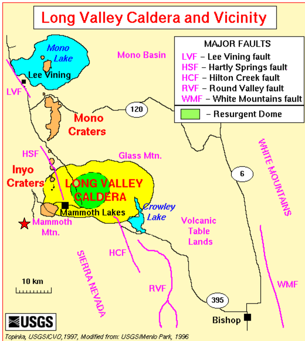
Figure 8. Long Valley Caldera and vicinity. Seismic unrest occurs in the Mono Lake – Long Valley area on a regular basis, and is monitored by the Long Valley Observatory. The red star (not to scale) represents the approximate location of Devils Postpile National Monument. Modified from U.S. Geological Survey graphic, available at: http://vulcan.wr.usgs.gov/Volcanoes/LongValley/Maps/map_long_valley.html . Accessed November 2009.
