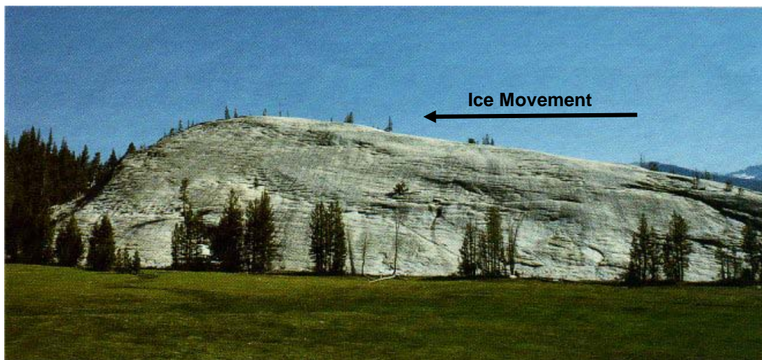
Figure 11. Pothole Dome, a large roche moutonnée in Yosemite National Park. Glaciers shaped Pothole Dome; ice moved from right to left over the bedrock surface (arrow). Plucking occurred on the downstream side; grinding and polishing occurred on the upstream side. U.S. Geological Survey photograph from Huber (1987), available at: http://pubs.er.usgs.gov/usgspubs/b/b1595 . Accessed November 2009.
