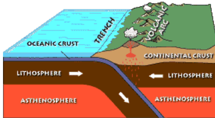
A) Oceanic-continental convergence (Andean-style, or Cascadian-style, subduction).
