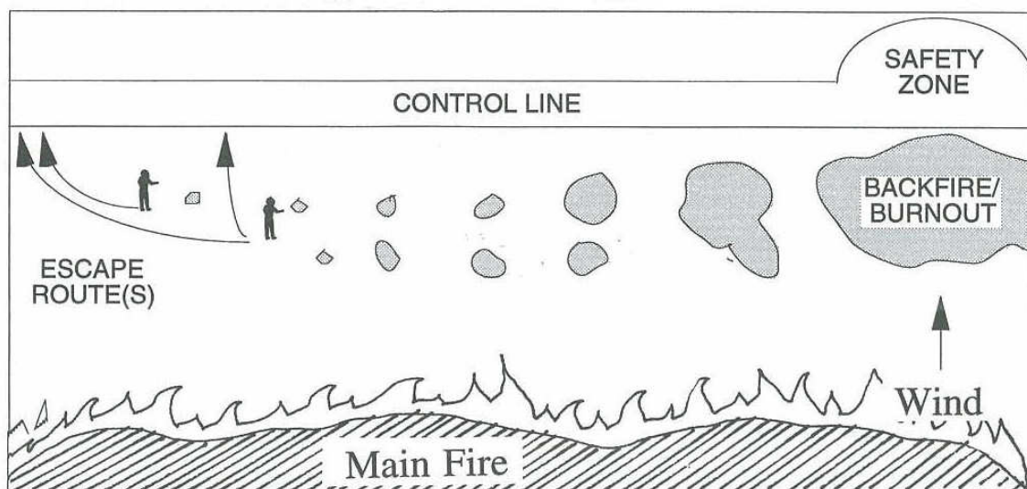
Figure 16 – Spot Firing
