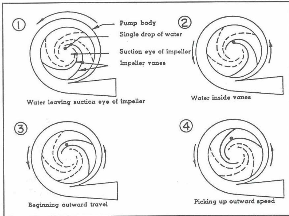
Figure 1 – Centrifugal Pump
