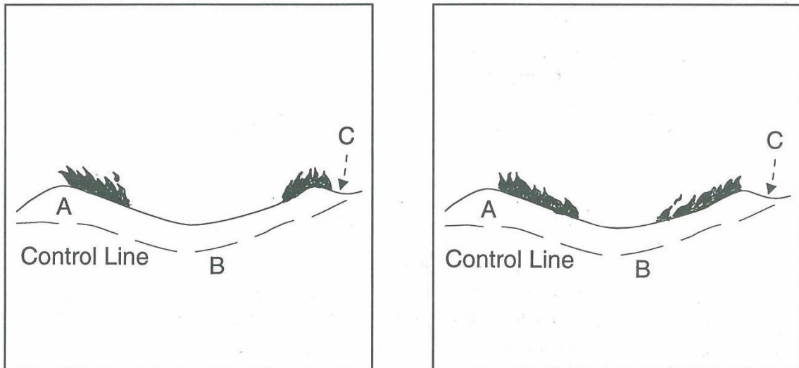
Figure 24 – Firing Saddles
