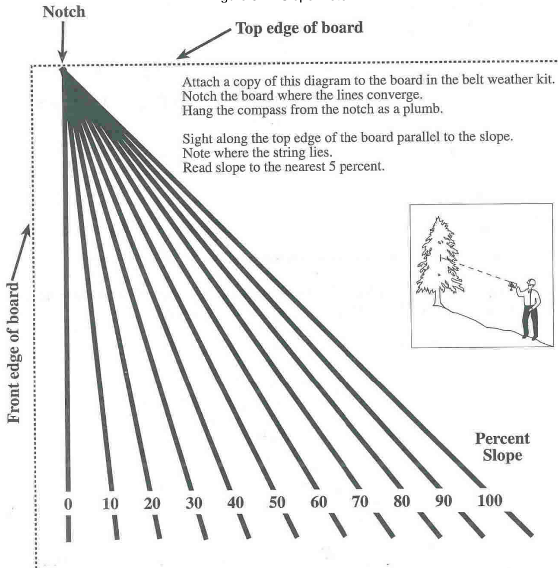
Figure 3 – Slope Meter
