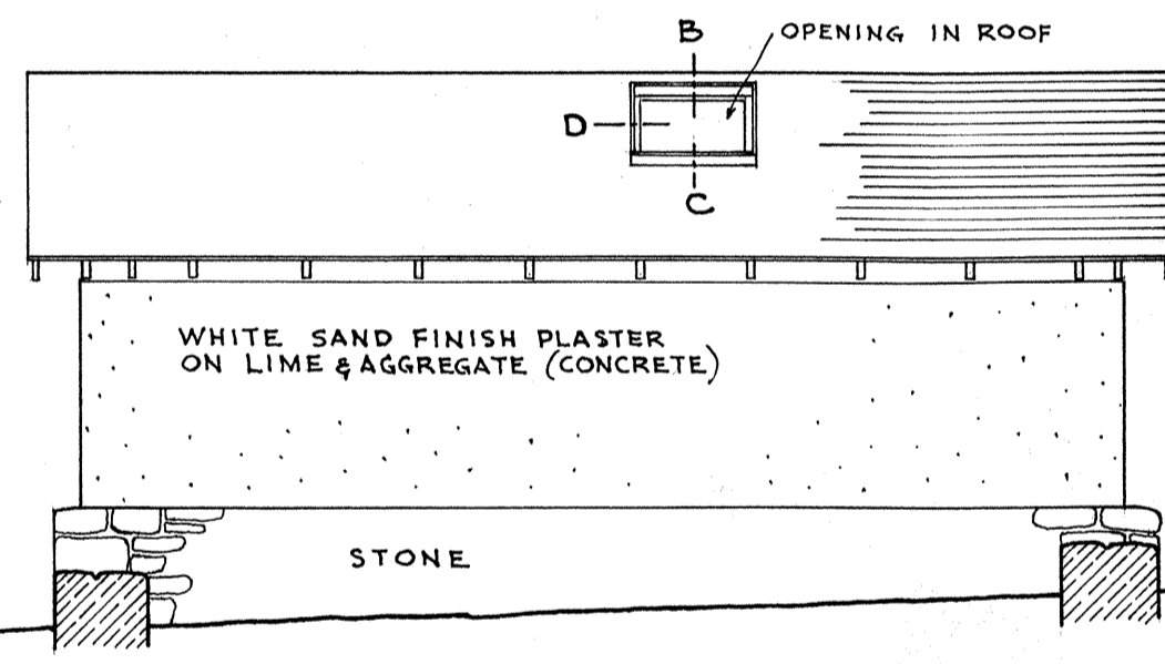
SOUTHEAST ELEVATION SCALE 1/4"=1'-0"
