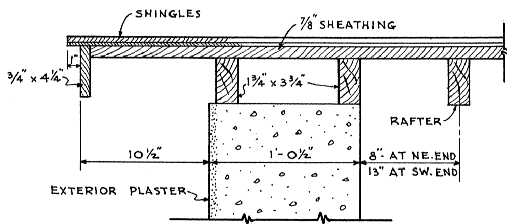
DETAIL OF RAKE SCALE 1 1/2"=1'-0"
