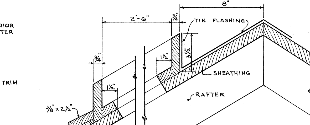
SECTION "B"
