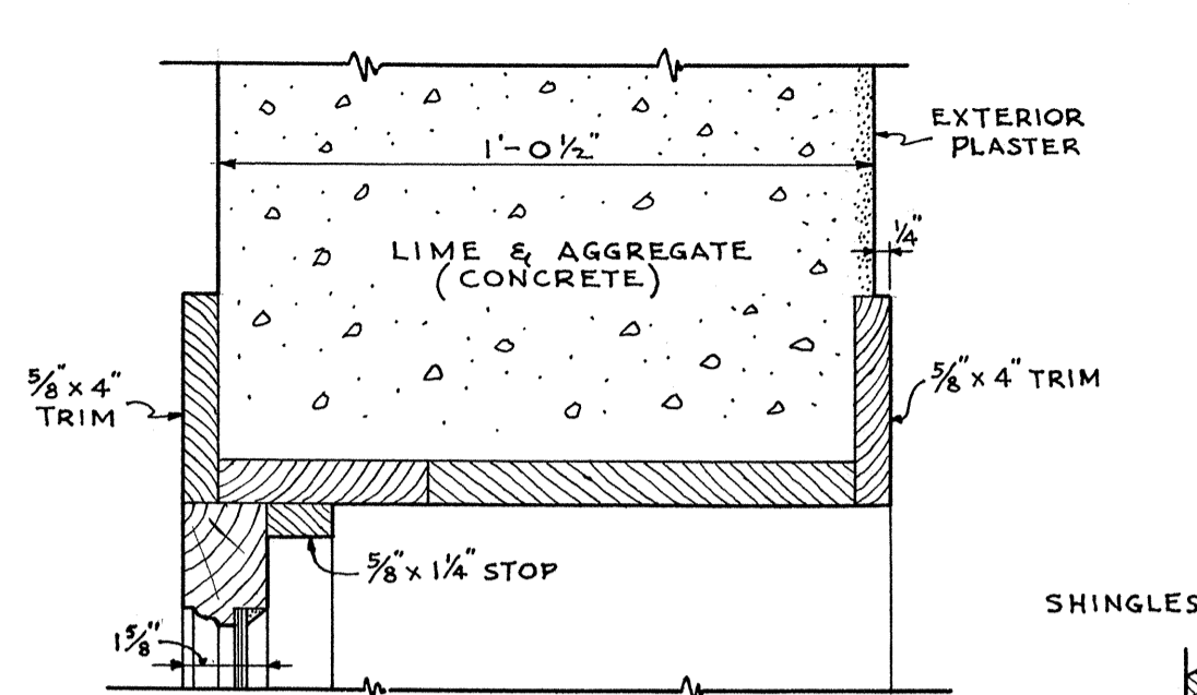
HEAD JAMB & SILL SIMILAR WINDOW DETAILS SCALE 3"=1'-0"
