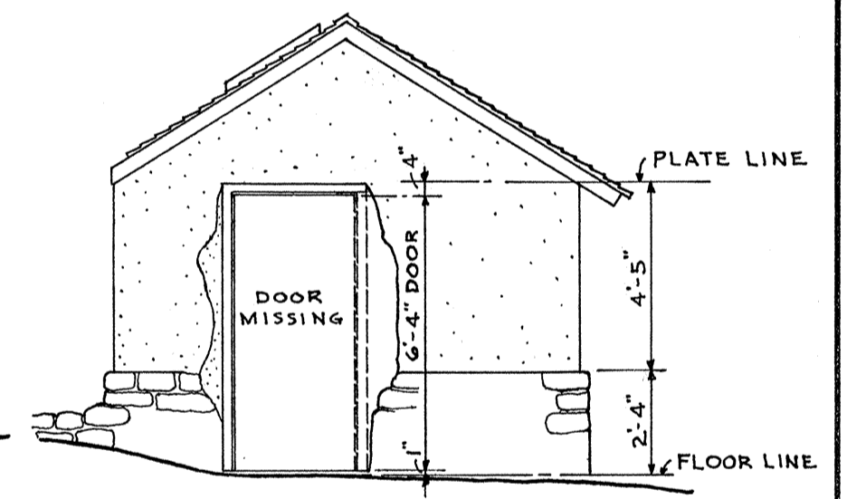
NORTHEAST ELEVATION
