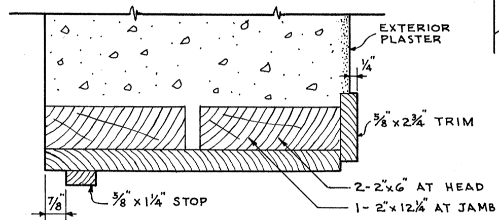
HEAD JAMB SIMILAR SILL MISSING DOOR DETAIL SCALE 3"=1'-0"
