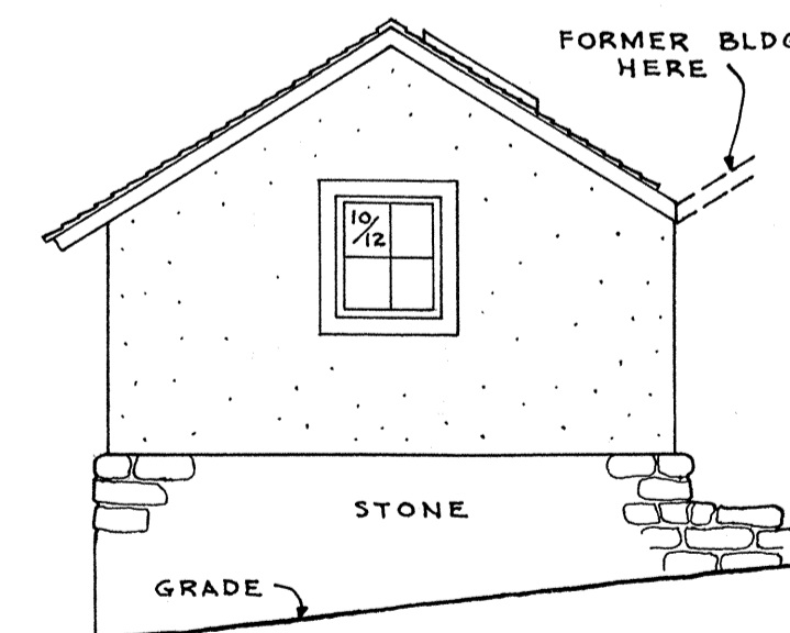
SOUTHWEST ELEVATION SCALE 1/4"=1'-0"
