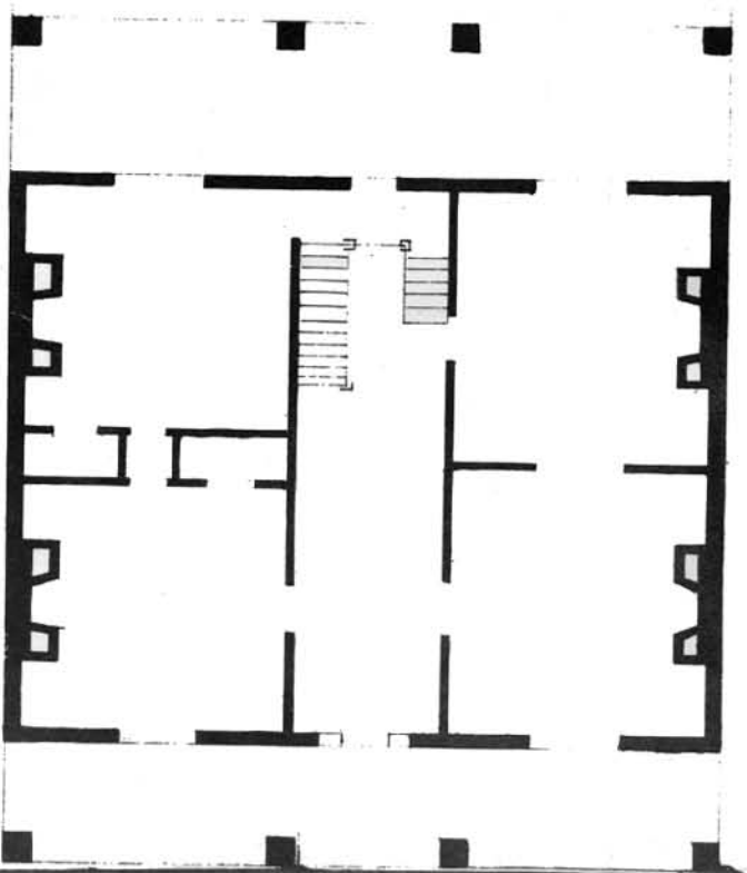
Plan for Commanding Officer's Quarters Fort Scott Quarters were never built. PLATE 1
