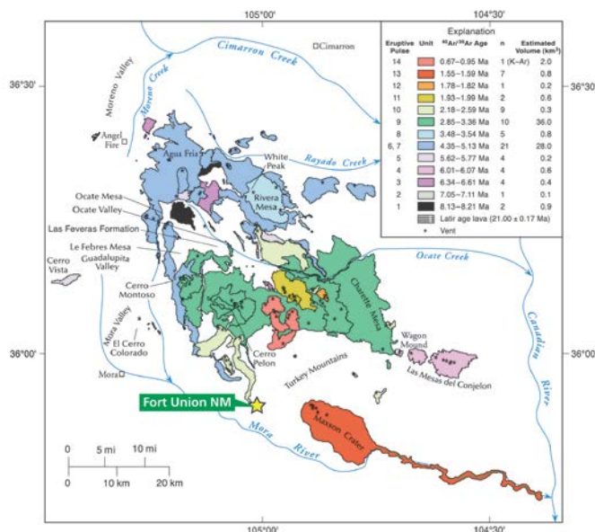
Figure 19. Lava flows of the Ocaté volcanic field. The Ocaté volcanic field erupted in 14 pulses, as shown on the figure. Olmsted and McIntosh (2004) radiometrically dated the lava flows using argon-40 ( ^{40}\text{Ar} ) / argon-39 ( ^{39}\text{Ar} ). The legend indicates the range of ^{40}\text{Ar}/^{39}\text{Ar} ages and the estimated volumes for each eruptive pulse. n = number of samples dated by Olmsted and McIntosh (2004). The flows closest to Fort Union National Monument are from eruptive pulse 10. Graphic from Olmsted and McIntosh (2004).
