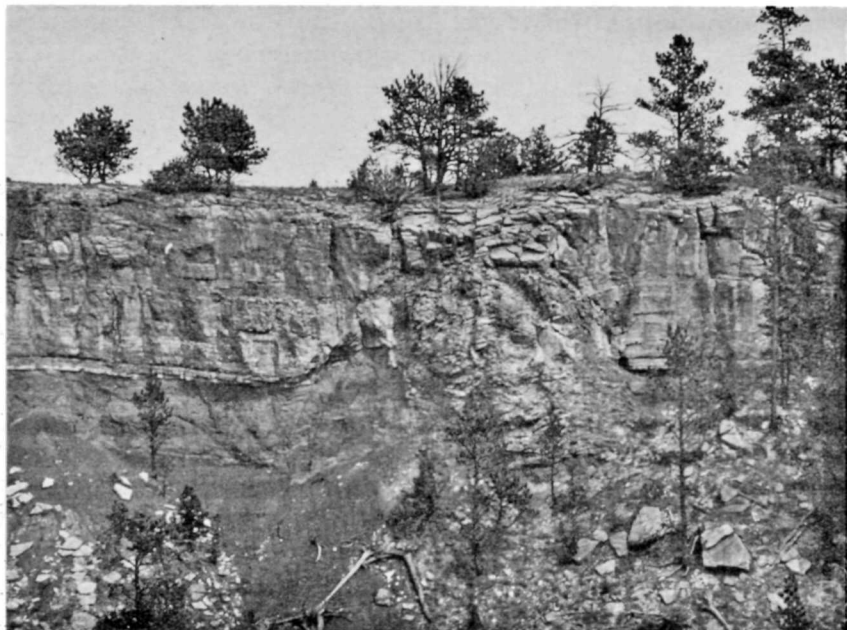
FIGURE 51.—Small breccia pipe that penetrates the Minnekahta Limestone in the SE \frac{1}{4} sec. 25, T. 5 S., R. 1 E. Small normal faults cut Opeche-Minnekahta contact at left side of pipe.
