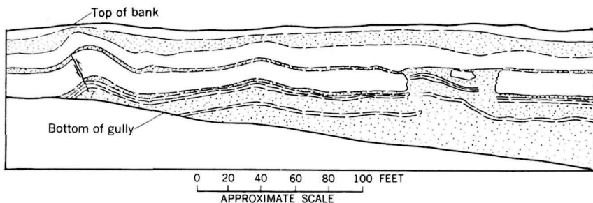
FIGURE 55.—Deformed gypsum beds in the Spearfish Formation. Stippled areas are siltstone. SW \frac{1}{4} sec. 26, T. 5 S., R. 1 E. Looking northeast.
