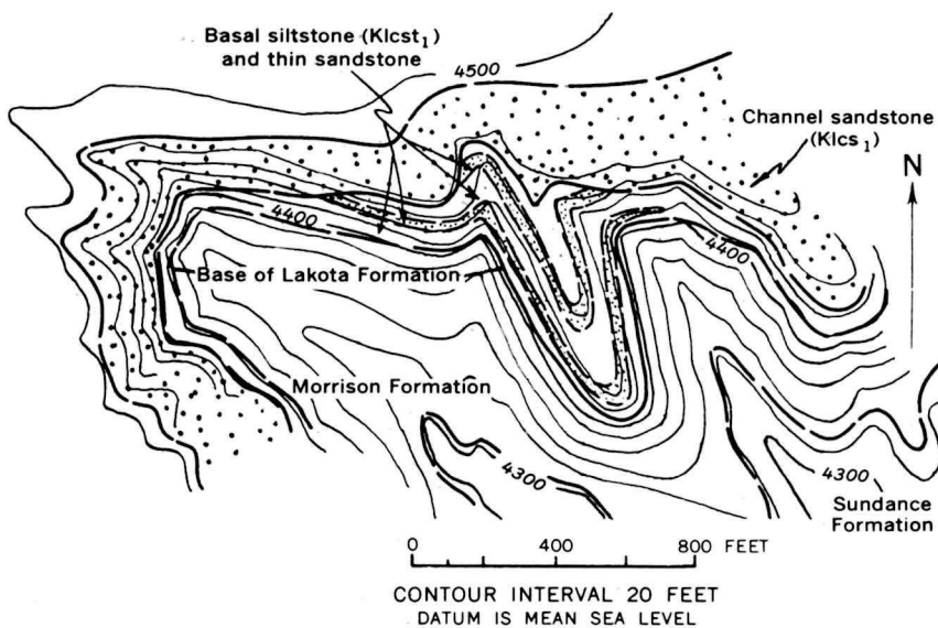
FIGURE 45.—Geologic map of part of secs. 28 and 29, T. 6 S., R. 2 E., showing the truncation of basal siltstone of the Lakota Formation by the overlying S_1 channel sandstone.
