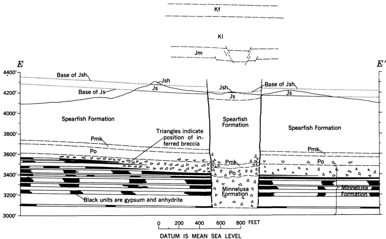
FIGURE 52.—Cross section E-E' of plate 20 showing inferred vertical extent of breccia pipe. Jsh, Hulett Sandstone Member of Sundance Formation; Js, Sundance Formation; Pmk, Minnekahta Formation; Po, Opeche Formation.
