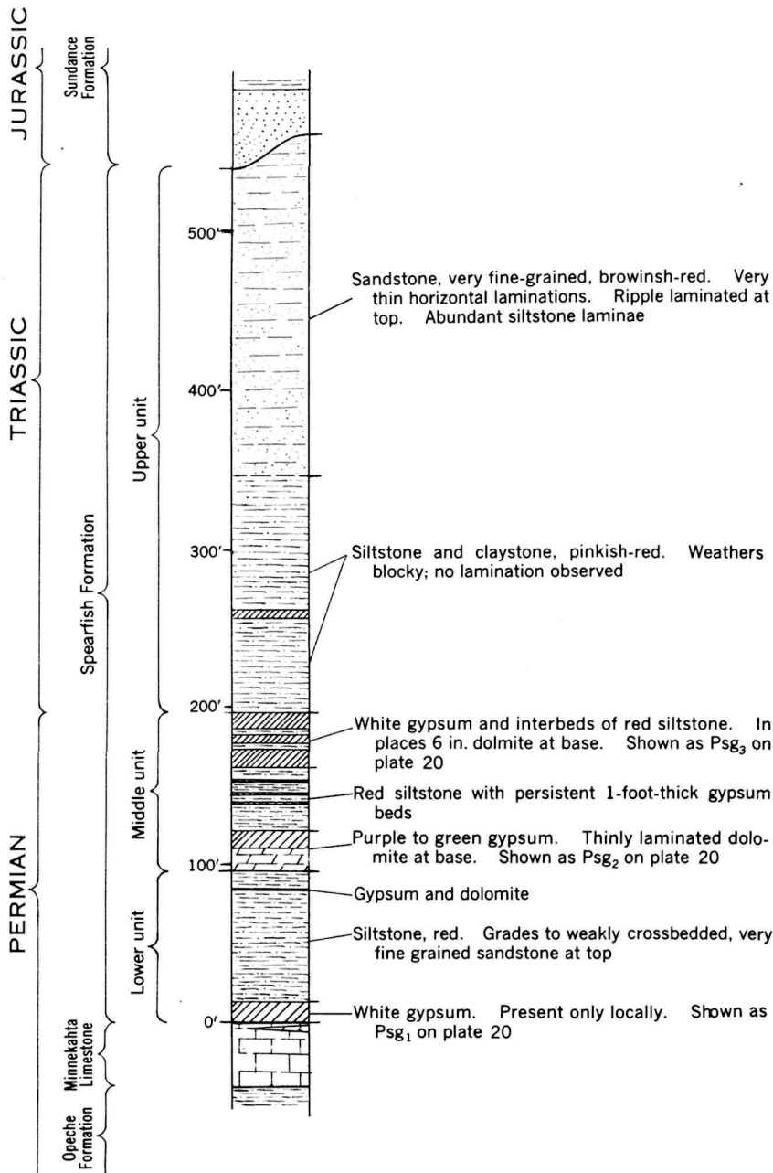
FIGURE 44.—Lithology of the Spearfish Formation.
