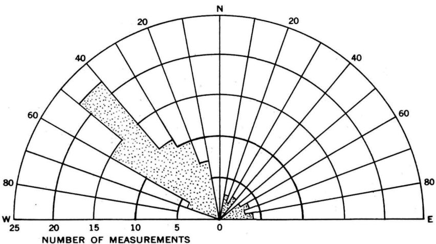
FIGURE 54.—Bearing of the axes of 92 minor folds in the Minnekahta Limestone, Jewel Cave SW quadrangle.
