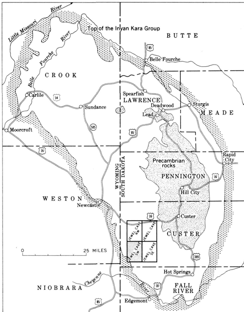
FIGURE 43.—Index map of the Black Hills showing the location of the Jewel Cave SW quadrangle, and some of the adjoining quadrangles.
