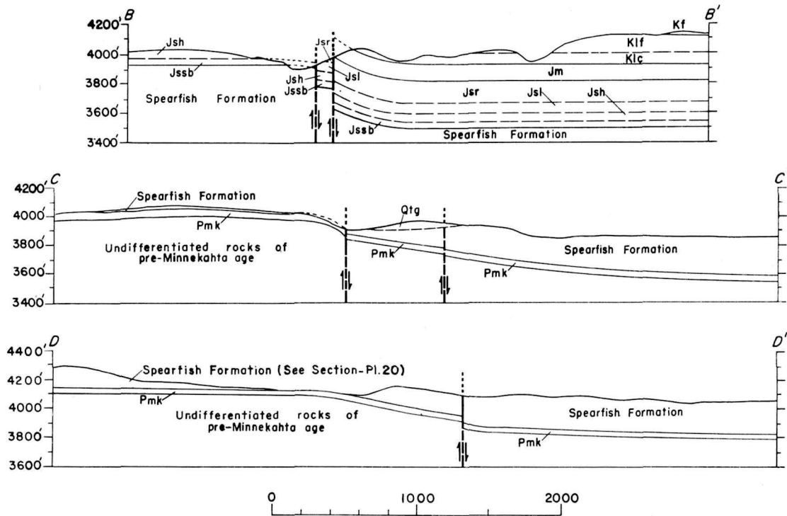
FIGURE 49.—Sections of the Dewey fault. Locations of sections shown on plate 20. Qtg, terrace gravel of Quaternary age; Kf, Fall River Formation; Klf, Fuson Member of Fall River Formation; Klc, Chilson Member of Lakota Formation; Jm, Morrison Formation; Jsr, Redwater Shale Member, Jsl, Lak Member, Jsh, Hulett Sandstone Member, Jssb, Stockade Beaver Shale Member, all of the Sundance Formation; Pmk, Minnekahta Limestone.
