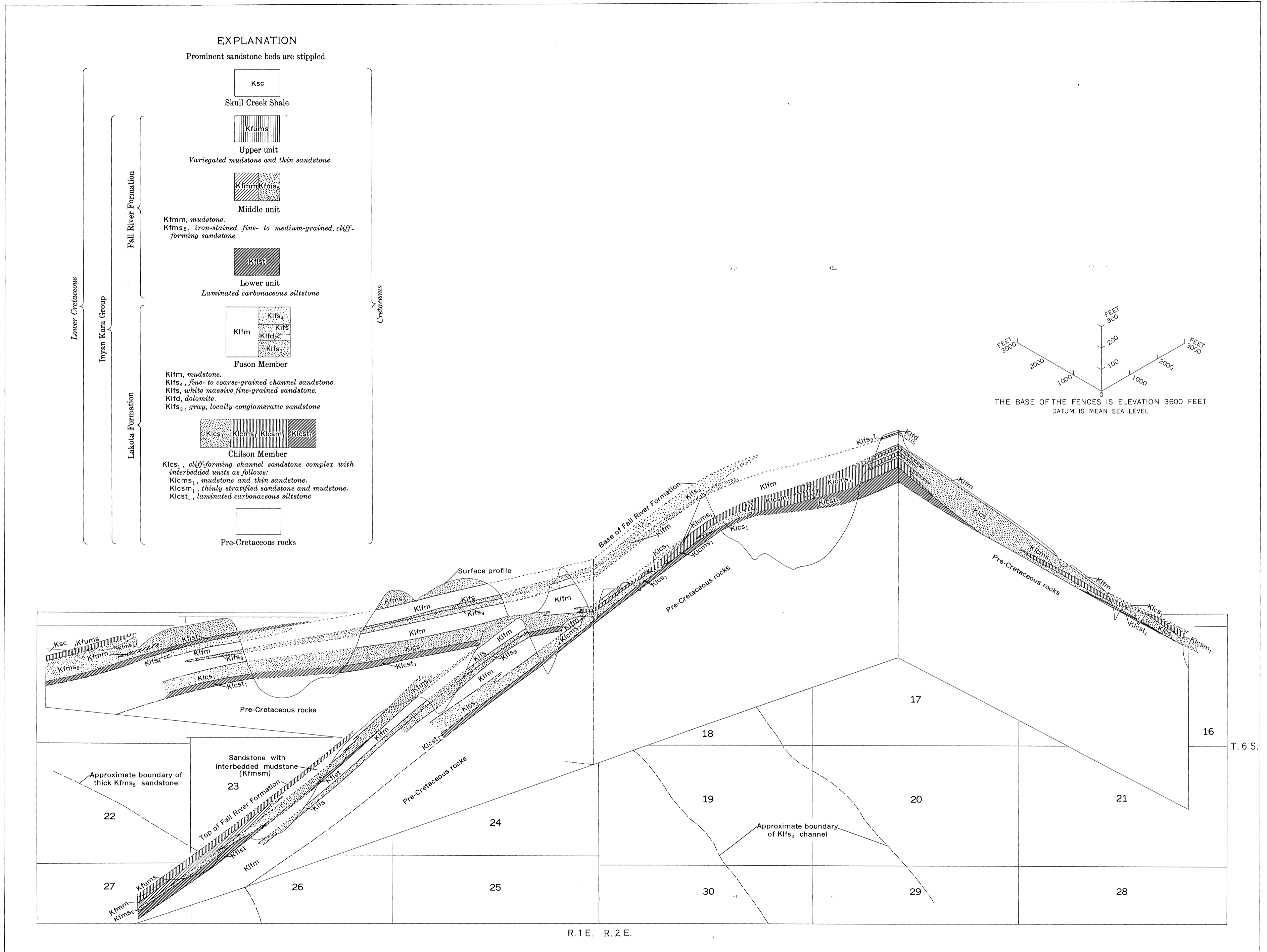
DIAGRAM SHOWING THE MAJOR LITHOLOGIC UNITS OF THE INYAN KARA GROUP IN THE SOUTHERN PART OF THE JEWEL CAVE SW QUADRANGLE
