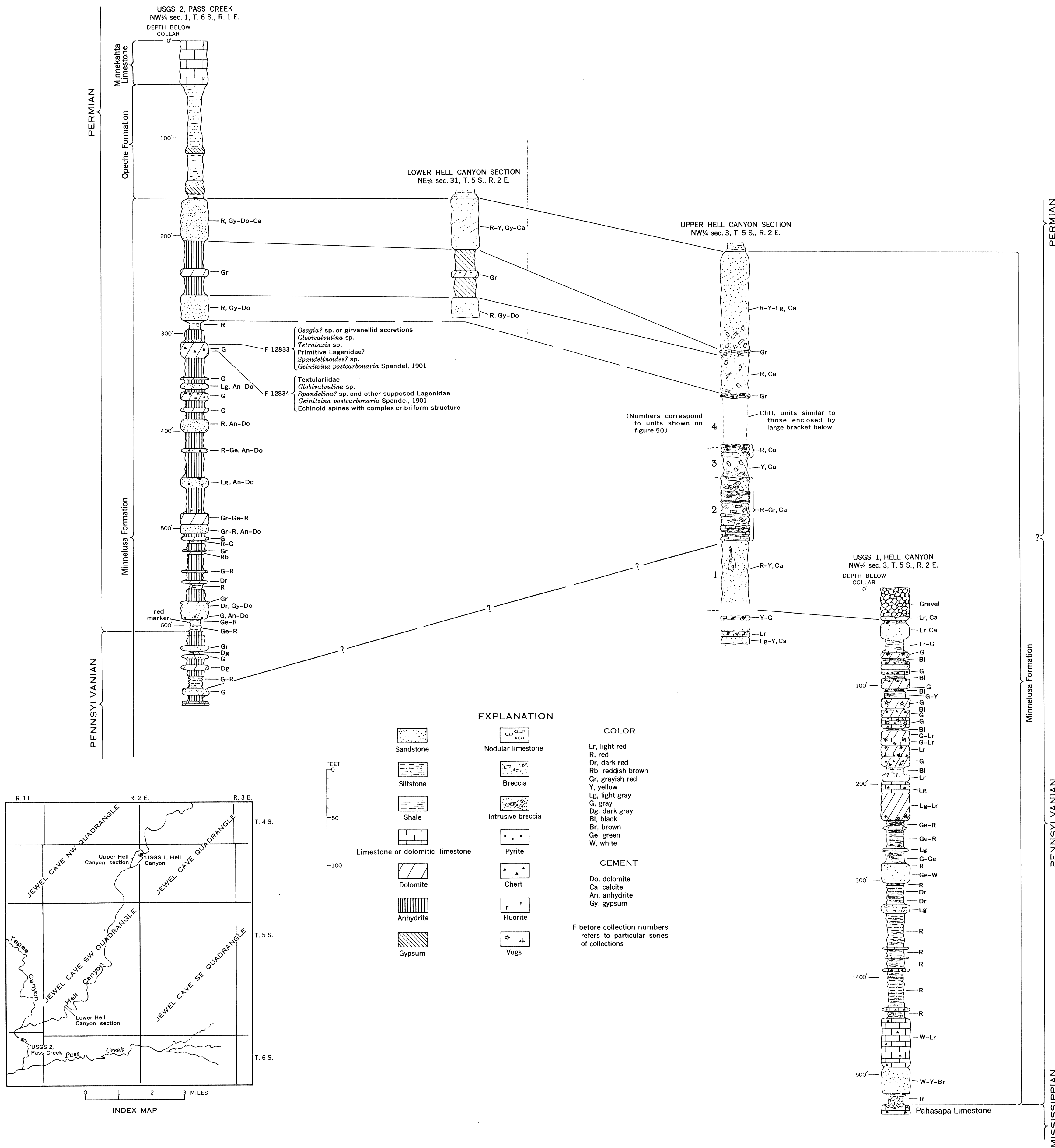
LITHOLOGY OF THE MINNELUSA FORMATION
