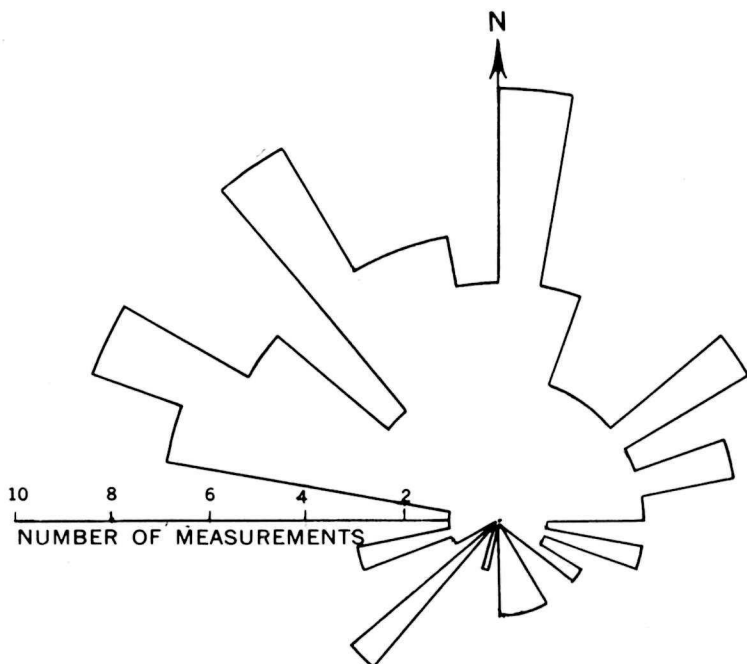
FIGURE 47.—Plot showing the direction of dip of 115 cross strata in the S_1 sandstone.
