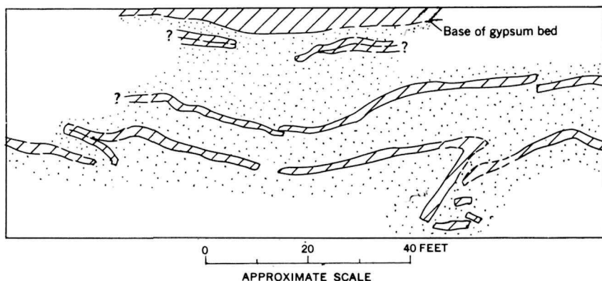
FIGURE 56.—Cross section of thin contorted gypsum beds underlying G_3 gypsum bed of the Spearfish. Stippled area is siltstone. NE \frac{1}{4} sec. 35, T. 5 S., R. 1 E. Looking northeast.
