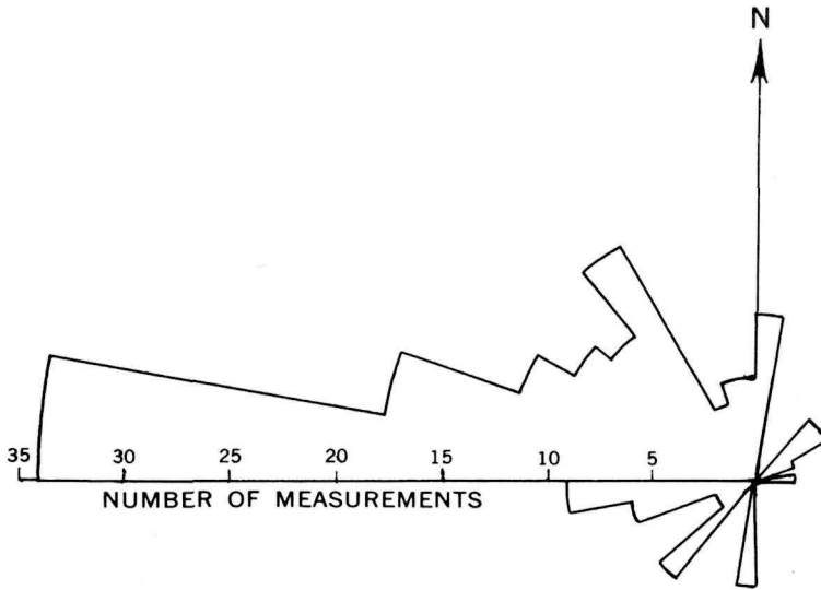
FIGURE 48.—Plot showing the direction of dip of 160 cross strata in the S_5 sandstone.
