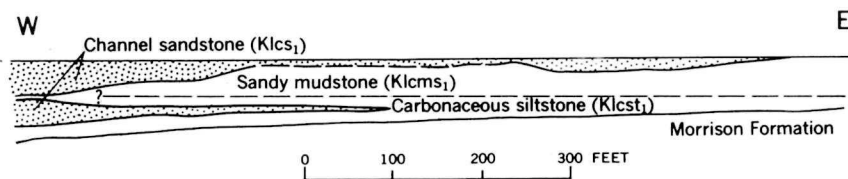
FIGURE 46.—Diagrammatic cross section along the boundary of secs. 18 and 19, T. 6 S., R. 2 E., showing interfingering of the S_1 channel sandstone and carbonaceous siltstone.
