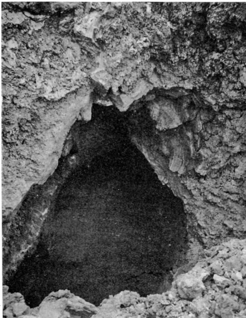
FIGURE 14.—View looking into the open chamber at the center of the 1949 cinder-and-spatter cone (cone 2), Mauna Loa, Hawaii. The flow-banded pahoehoe lining of the chamber is clearly visible, and at the top a dike extends upward through the cinder. Photograph by G. A. Macdonald.
