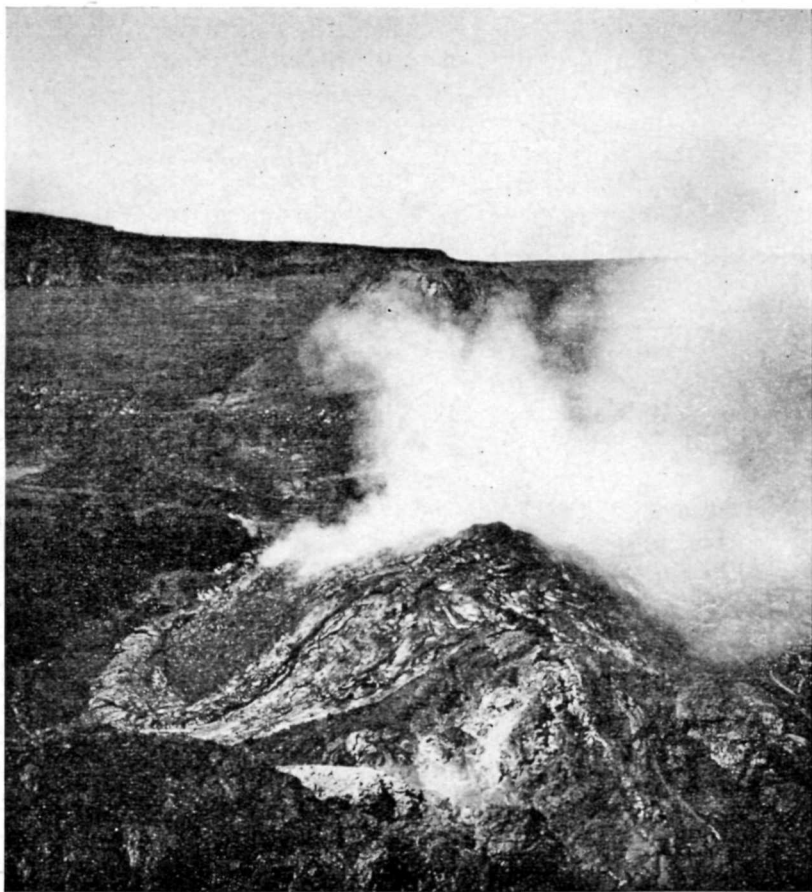
FIGURE 12.—Small cinder-and-spatter cone (cone 2), Mauna Loa, Hawaii, seen from the summit of the larger pumice-and-cinder cone to the southwest on May 7, 1949. One horn of the breached pumice cone is visible on the left. The cinder-and-spatter cone is partly veneered with lava flows. The 1940 cone is visible in the background. Photograph by John Bonsey.
