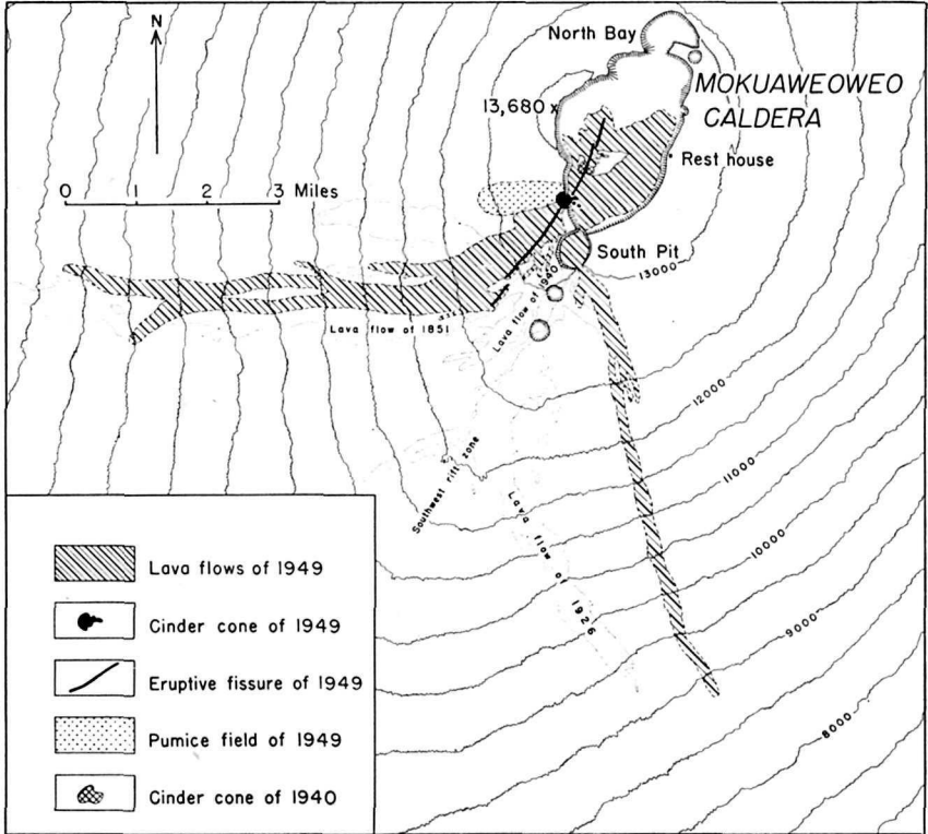
FIGURE 2.—Map showing the approximate distribution of the lavas and the location of the vents of the 1949 eruption of Mauna Loa, Hawaii.
