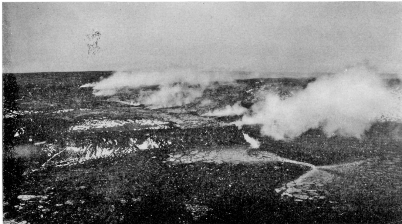
FIGURE 4.—Southwest edge of Mokuaweoweo caldera, Mauna Loa, Hawaii, on the morning of January 7, 1949, showing the eruptive fissure crossing the wall of the caldera and extending on down the outer slope of the mountain. Lava fountains are playing from the fissure at the base of the caldera wall and at several points along the fissure beyond. At the right a new lava flow is flowing northward onto the caldera floor, and at the left another lava stream is pouring into South Pit. Official photograph of the United States Navy.
