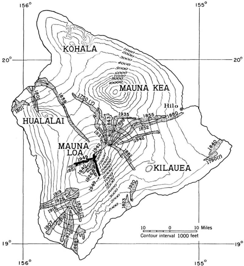
FIGURE 1.—Map of the island of Hawaii, showing the position of the 1949 lava flows (solid black) in relation to other historic flows (stippled) of Mauna Loa and Kilauea.
