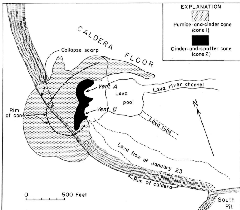
FIGURE 7.—Sketch map of the area in the vicinity of the 1949 cinder cone at the southwest edge of Mokuaweoweo caldera, Mauna Loa, Hawaii, in February, at the end of the period of large lava fountains.
