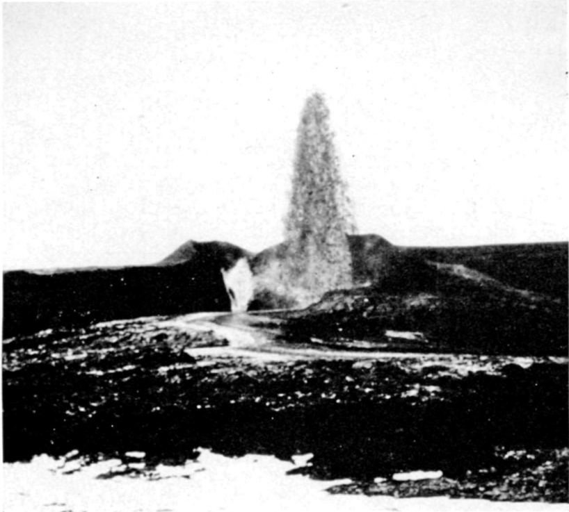
FIGURE 6.—Lava fountains at the southwest edge of Mokuaweoweo caldera, Mauna Loa, island of Hawaii, on January 21, 1949. The higher fountain is playing to a height of about 500 feet. Behind and to the left of it a smaller fountain plays from the fissure in the caldera wall. The fountains are building a large cone of cinder and pumice. A lava flow issues from the breached crater of the compound cone. Photograph by F. A. Hjort, National Park Service.
