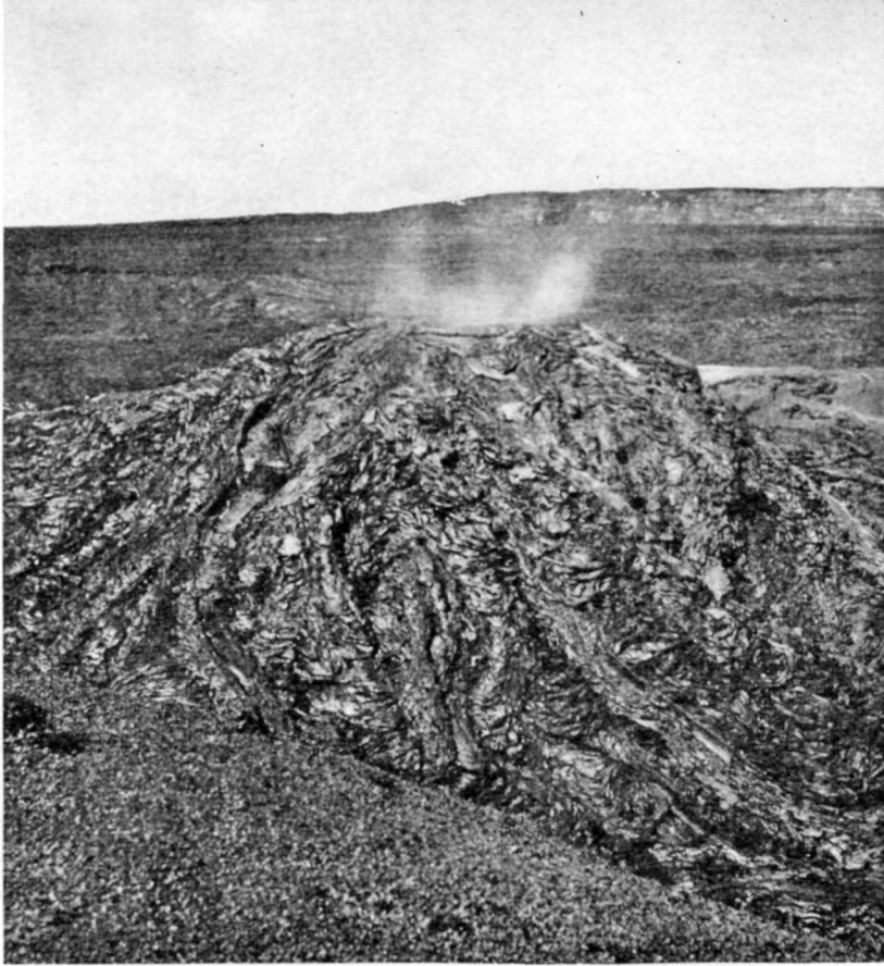
FIGURE 11.—The 1949 lava cone (cone 3), Mauna Loa, Hawaii, seen from the top of the caldera wall to the southwest on May 7. Mokuaweoweo caldera is in the background. Photograph by John Bonsey.
