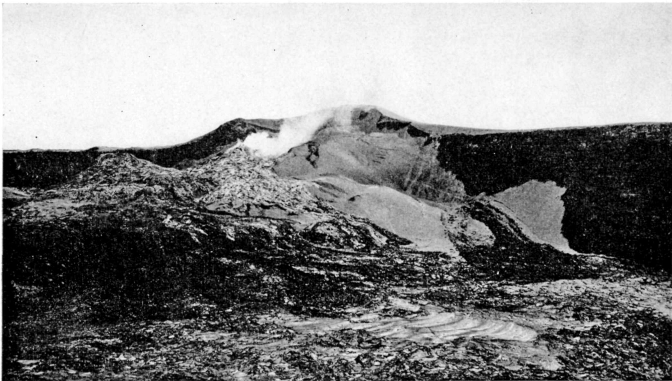
FIGURE 8.—Cone area of the 1949 eruption at the southwest edge of Mokuaweoweo caldera, Mauna Loa, Hawaii, seen from the 1940 cone on June 3, 1949. In the background the large cinder-and-pumice cone rests against and on top of the caldera wall and has partly collapsed. Within its crater the small cinder-and-spatter cone (cone 2), largely covered by lava flows, is fuming strongly. Farther to the left the lava cone (cone 3) is visible. Photograph by J. B. Orr.
