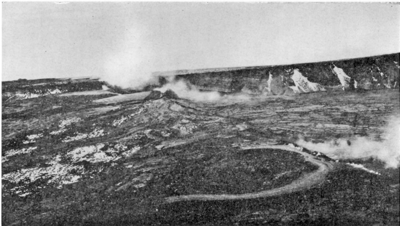
FIGURE 3.—Mokuaweoweo caldera, Mauna Loa, island of Hawaii, looking southwestward on the morning of January 7, 1949. The northern fountain chain and the lava flow leading eastward from it are in the right foreground. In the middle distance the eruptive fissure cuts through the 1940 cinder cone, which can be seen fuming strongly. Official photograph of the United States Navy.
