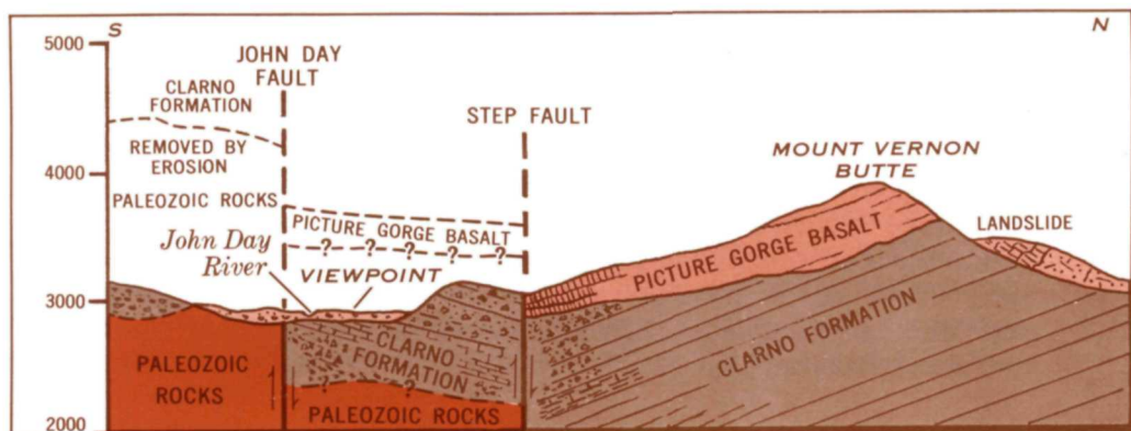
Fig. 2.—Mount Vernon Butte and diagram of faulting on south slope.
