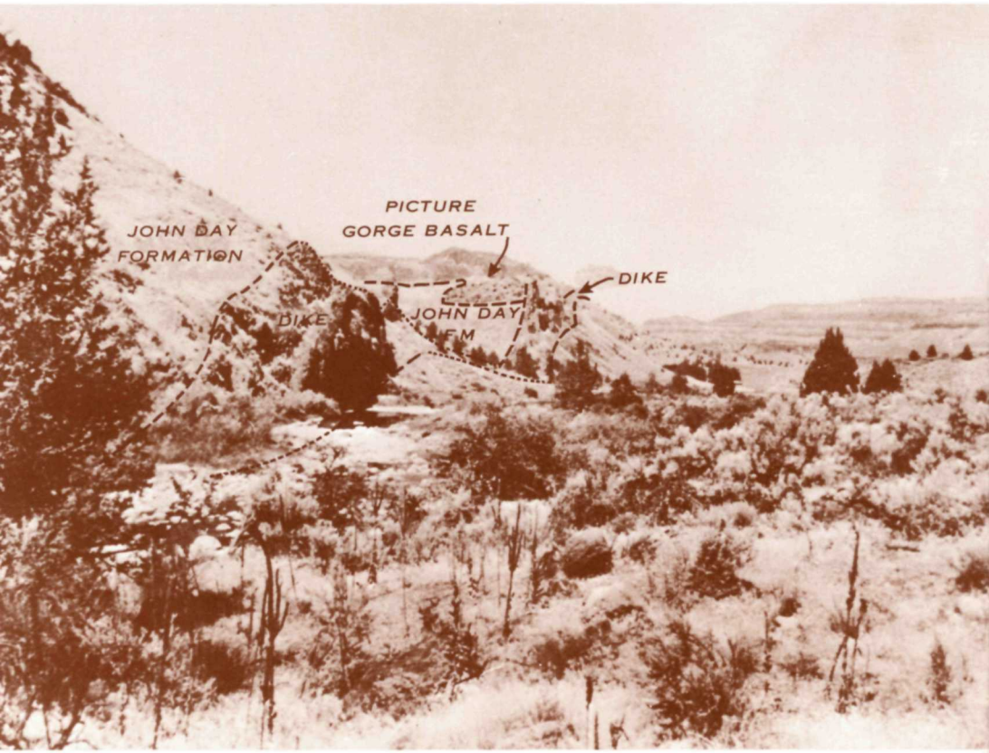
Fig. 8.—Basalt dike 2 miles south of Kimberly.
