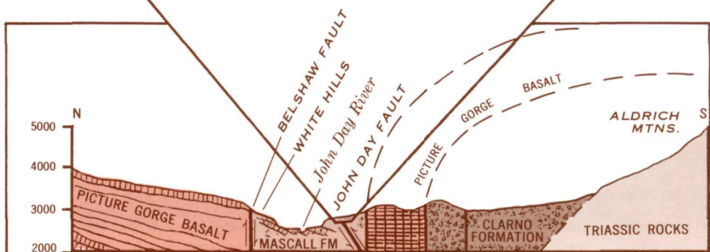
Fig. 3.—John Day fault in Mascall Formation at the mouth of Fields Creek and its relation to the structure of the John Day River valley.
