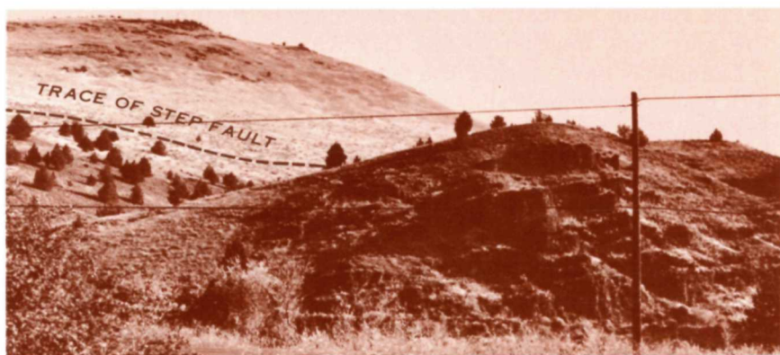
Fig. 2.—Mount Vernon Butte and diagram of faulting on south slope.
