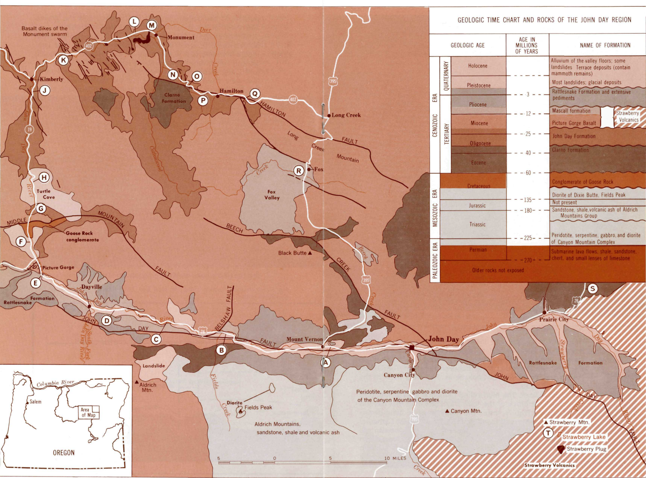
Fig. 1.—Geologic map of the John Day Country showing road log route.
