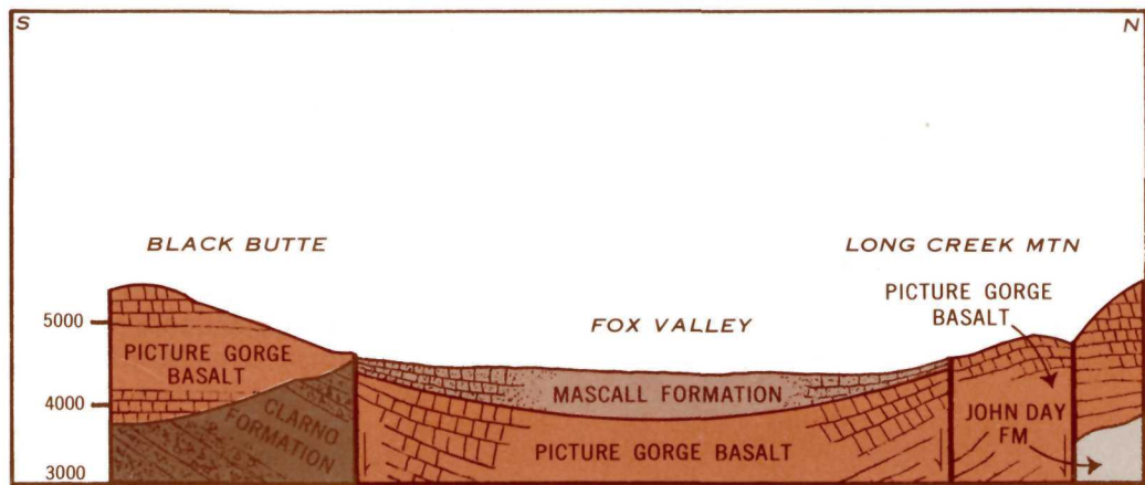
Fig. 12.—North-south section of Fox Valley, showing faulted basin structure.
