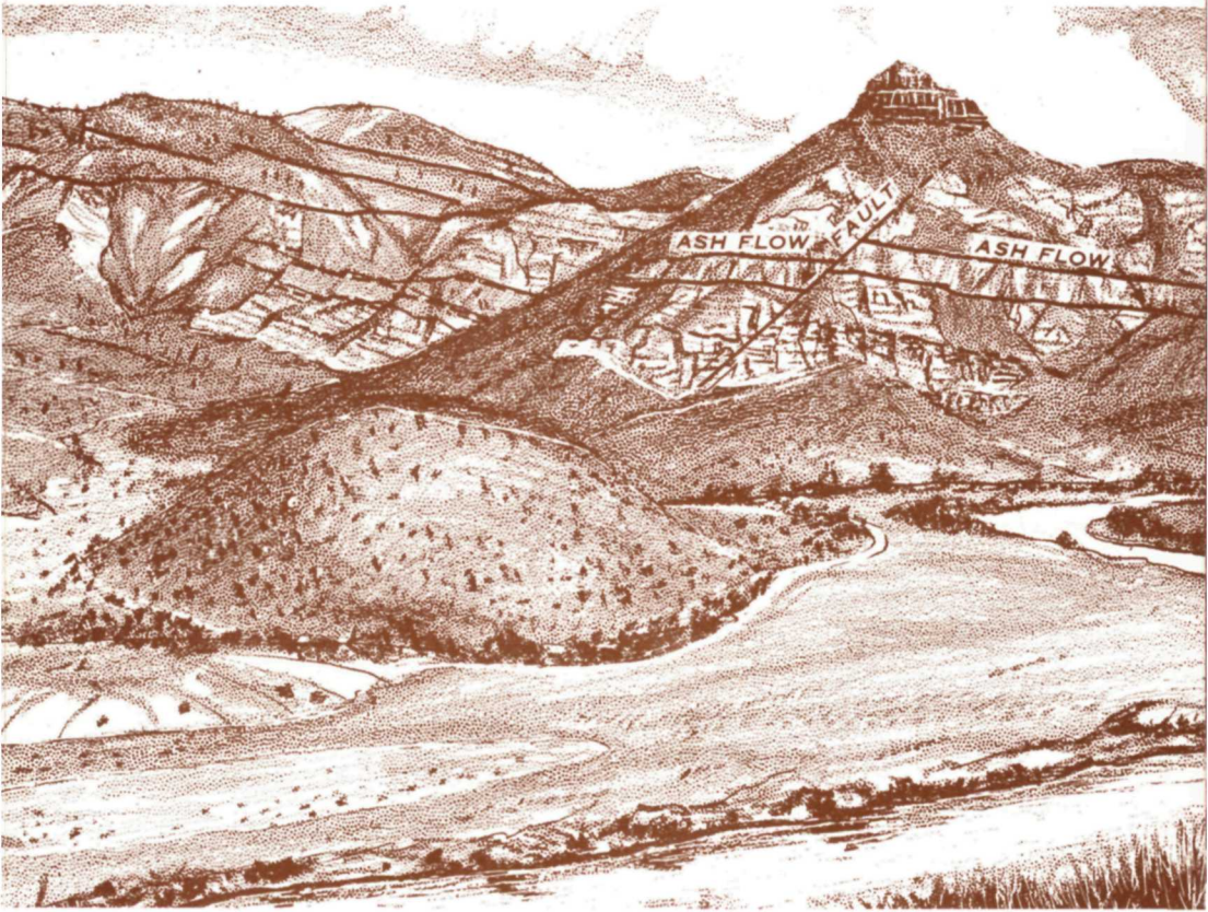
Fig. 6.—Sheep Rock from Sheep Rock Overlook.
