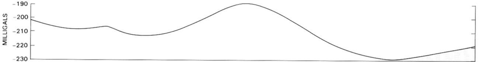
BOUGUER GRAVITY ANOMALY PROFILE
