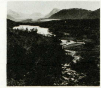
FOREST GROWTH QUICKLY INVADES AREAS FORMERLY COVERED BY GLACIAL ICE.
