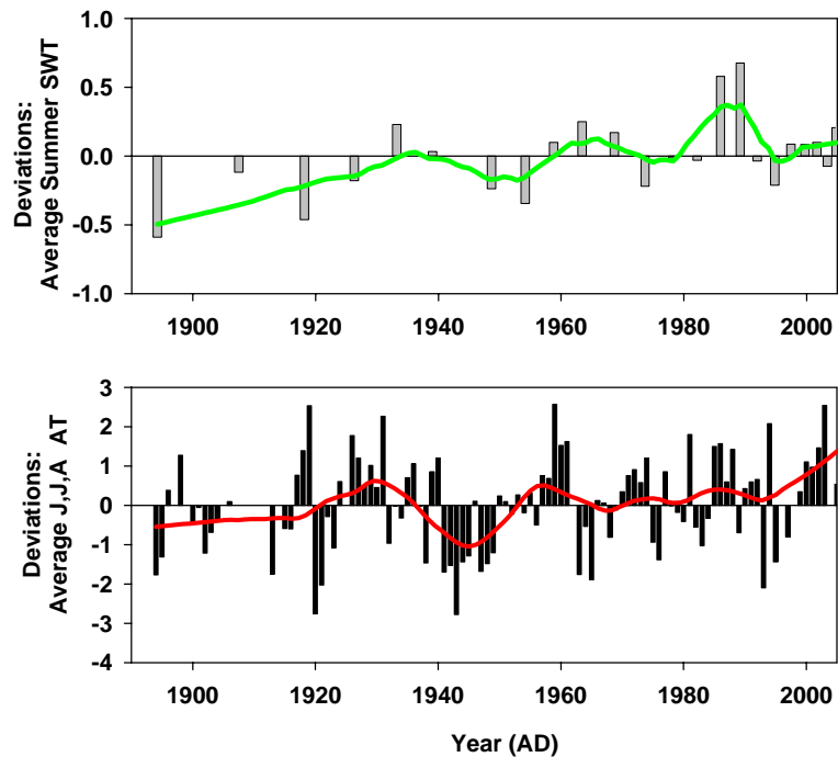
Figure 1. Chironomid-based surface water temperature reconstruction for Stella Lake spanning the interval AD 1895 – 2005 (based on 210 Pb analyses). This figure depicts the deviations of the chironomid-based surface water temperature estimates from the average surface water temperature from AD 1895 – 2005 and the deviations of air temperature from long-term average air temperature over the period AD 1895 – AD 2005 for Austin, Nevada (NCDC, 2006). The heavy, solid lines represent a LOWESS smoother.
