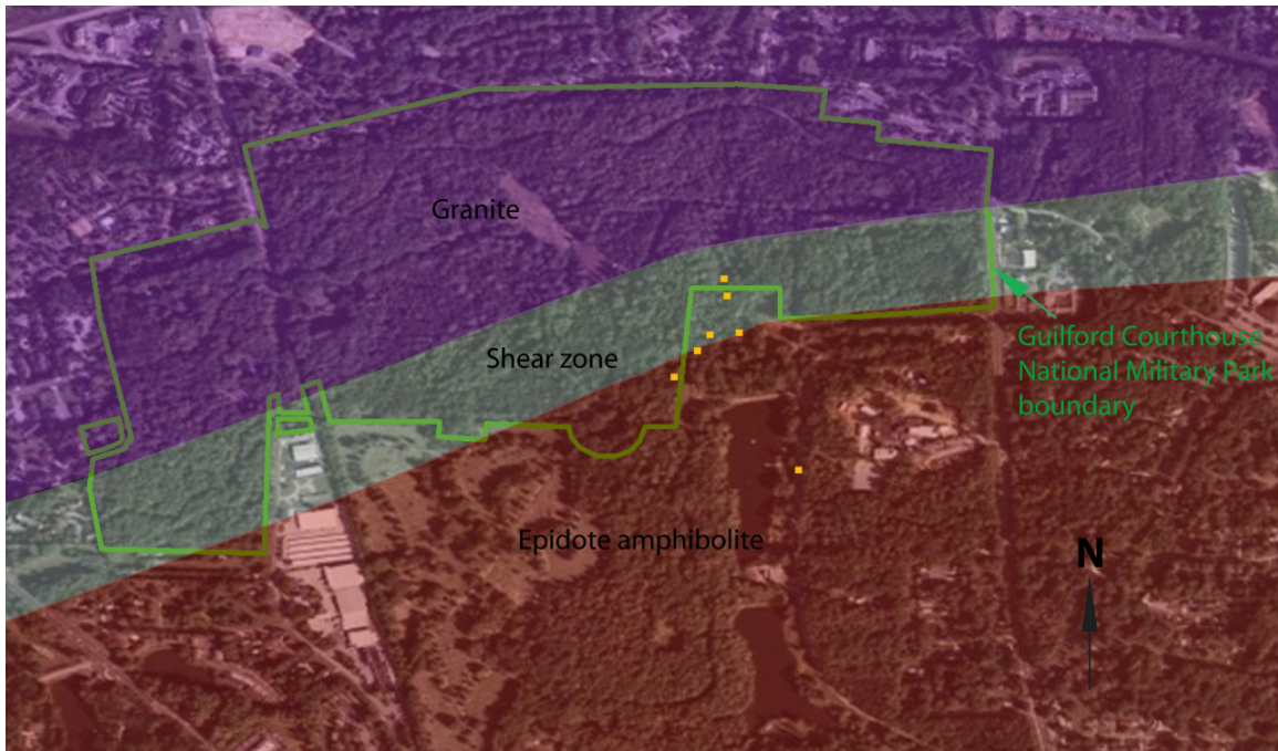
Figure 8. Aerial view of Guilford Courthouse National Military Park with recent geologic mapping superimposed. Shear zone between granitic rocks typical of the Charlotte belt and amphibolite rocks typical of the Carolina Slate belt runs directly through the park. Note the location of bedrock outcrops (yellow squares) within the park area. Mapping by Mininger and Nunnery (2001). Graphic by Trista L. Thornberry-Ehrlich (Colorado State University). Base map compiled by Jason Kenworthy (NPS Geologic Resources Division) from ESRI ArcImage Server, USA Prime Imagery.
