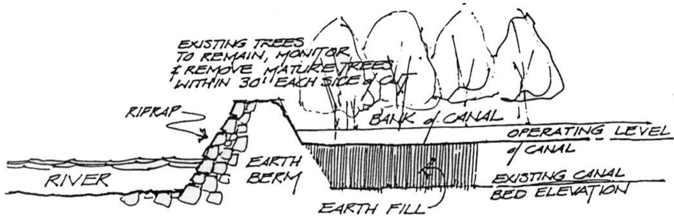
SECTION AT UPSTREAM ENTRANCE
