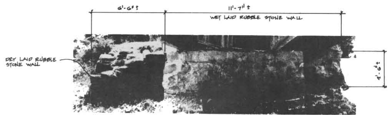
③ 11 FOOTBRIDGE AT FOUNDRY SITE ( SLUICEWAY ) SOUTH ELEVATION UNDER BRIDGE
