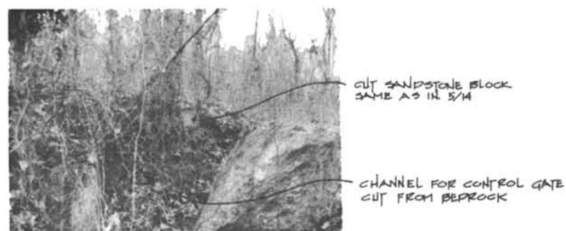
4 14 CONTROL GATE AT LOWER HOLDING BASIN ( EAST OF LOCK 2 ) VIEW LOOKING NORTHWEST
