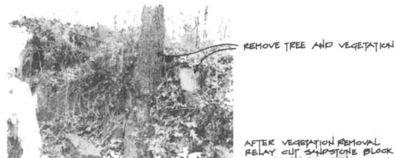
5 27 CONTROL GATE AT LOWER HOLDING BASIN ( EAST OF LOCK 2 ) VIEW LOOKING SOUTHWEST (PRIORITY 2C)
