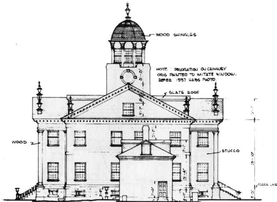
WEST ELEVATION SCALE: 3/32" = 1'-0"
