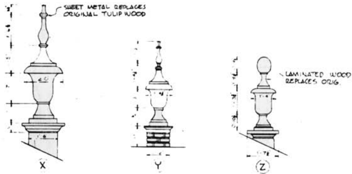
FINIAL DETAILS SCALE: 1/2" = 1'-0"
