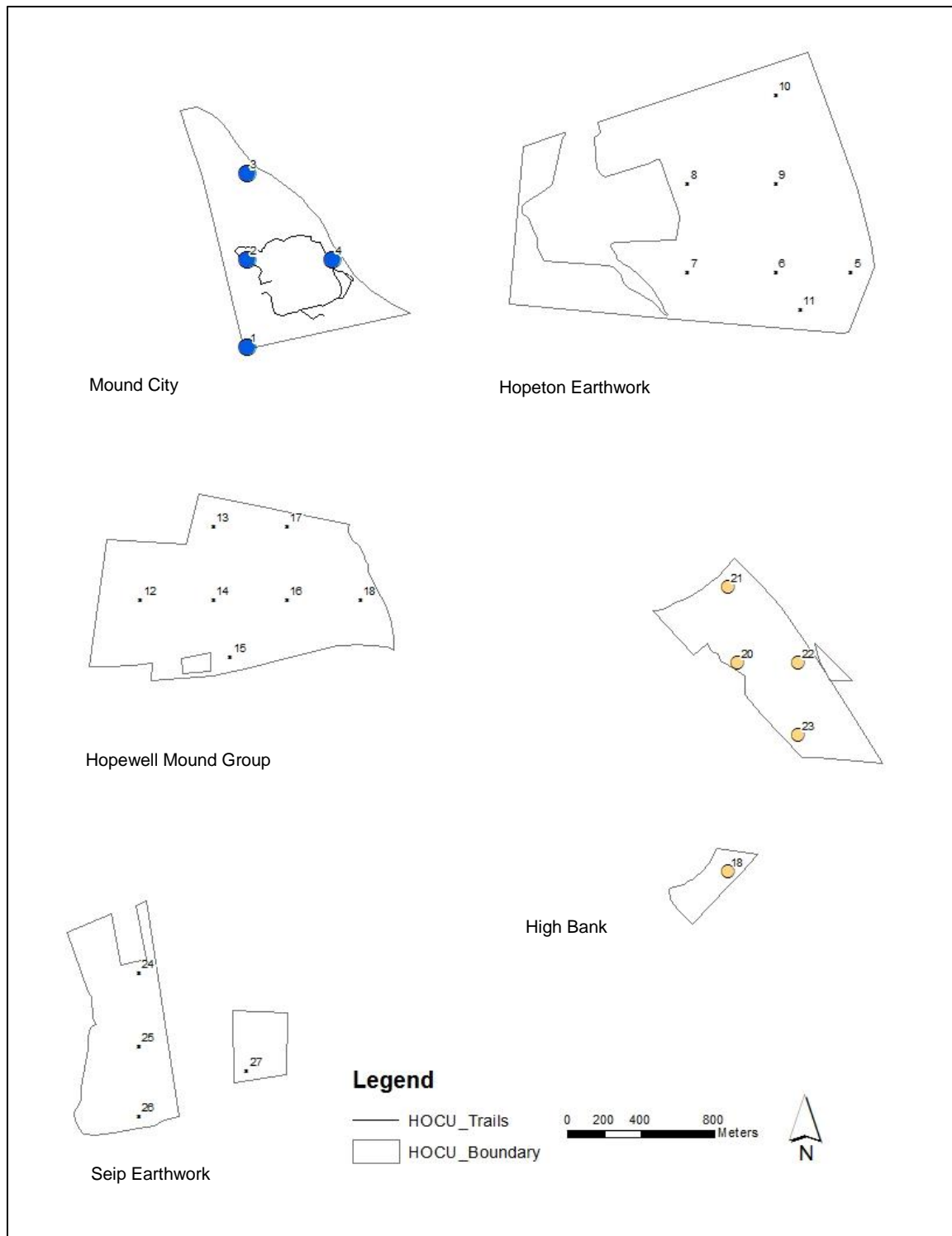
Figure 1. Areas of higher {gold (high) \square red (higher)} and lower {light blue (low) \square dark blue (lower)} than expected breeding bird species richness for plots on Hopewell Culture National Historical Park, Ohio in 2012.
