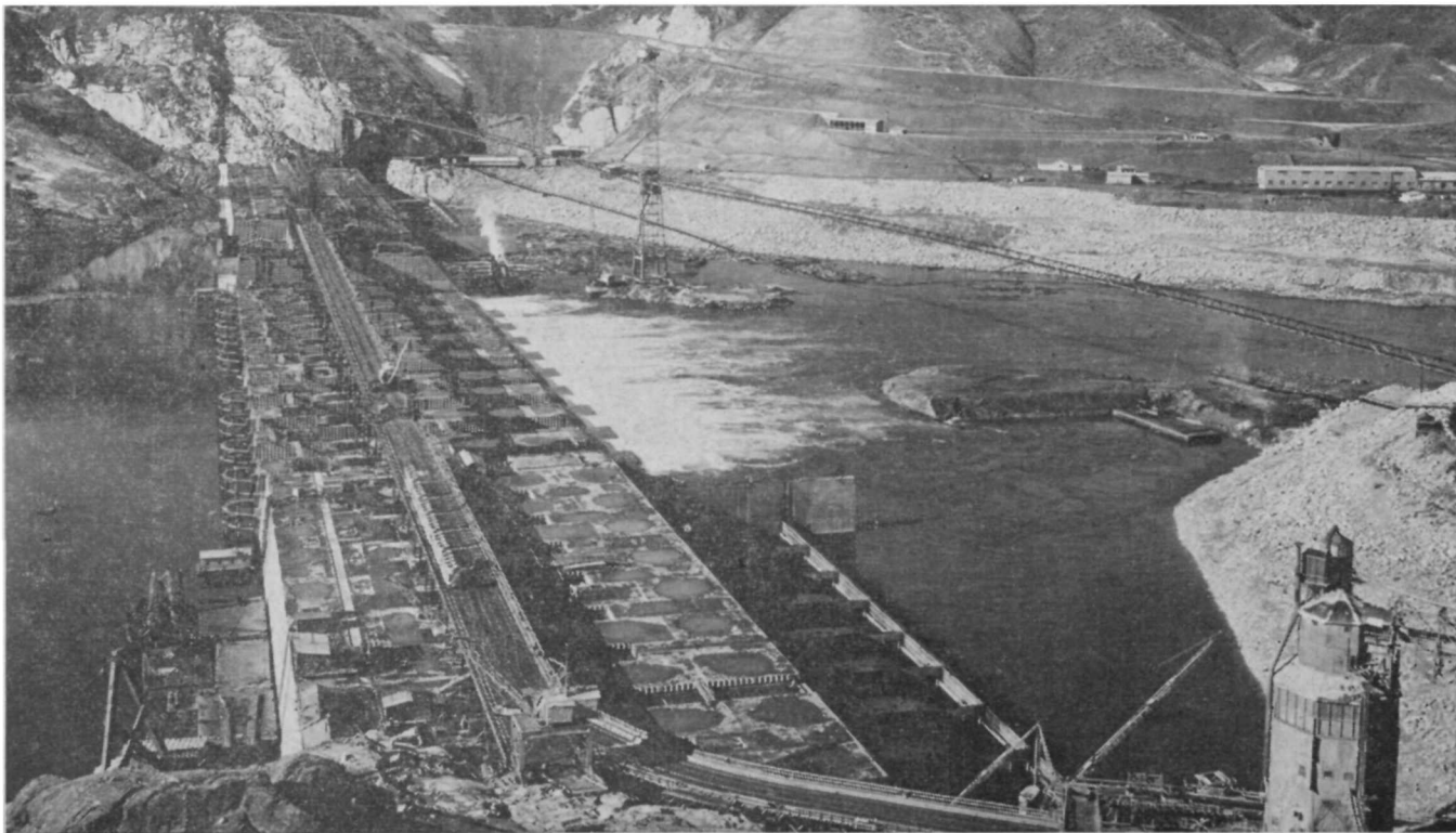
Grand Coulee Dam as taken over by Consoliated Builders, Incorporated, March 1938. Excavation in solia granite on West bank shows Dam will reach to within a few feet of roadway. Water now flows thru gaps in Dam over 1650-ft. Spillway. North coffer-dam used in diverting river shows below spillway in process of dismantling. Power-house foundations may be seen on either side of wings of spillway. Pumping plant foundation shows in granite to left of Dam.
