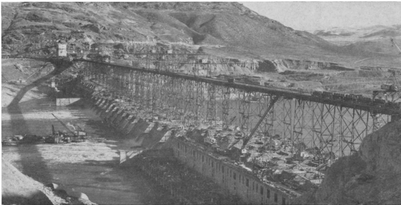
View from West side, March 1939. Water flows through 50-foot gaps at either end of spillway. Note white mixing plant, cranes 300 feet long, and concrete cars show on trestle. Present trestle supports will be imbedded in concrete. Another trestle of about same height needed to complete Dam.
