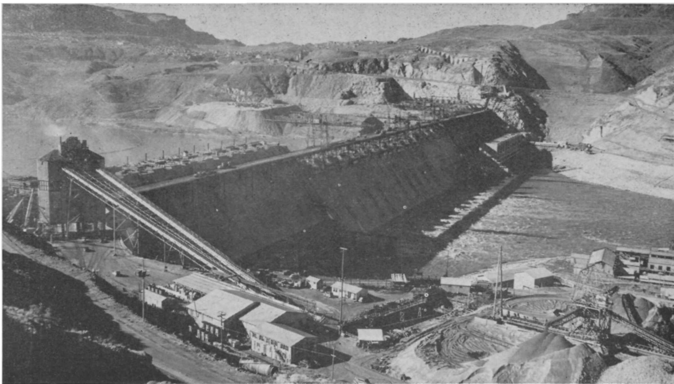
Construction March 1940. Concrete of Dam on ends rises above trestle on which concrete cars and jack-hammer cranes show. West power house is nearing completion on right end of Dam. Concrete mixer with conveyor belts shows on left end. Sand and gravel storage in lower right. Water above Dam finds outlet through conduits in base of spillway section.
