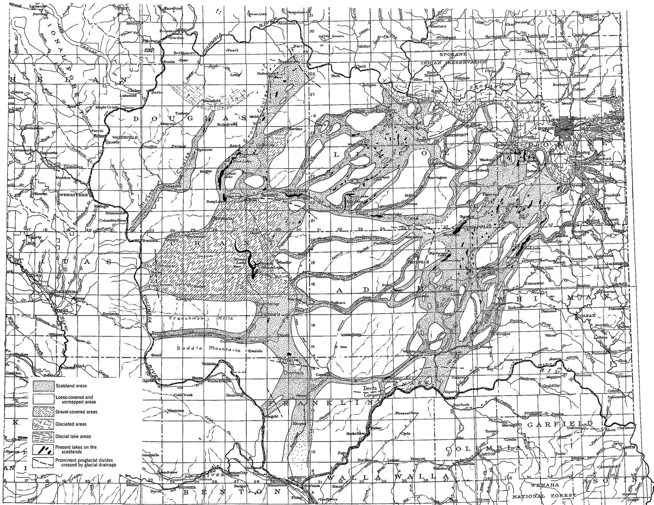
THE CHANNLED SCABLANS OF THE COLUMBIA PLATEAU AND THEIR ASSOCIATED FEATURES The small squares are townships and indicate the scale of the map
