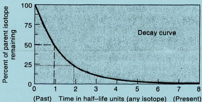
FIGURE 5.5 Simple arithmetic plot of a universal isotopic decay curve. After one half-life has elapsed, 50 percent of the original parent isotope remains; after two half-lives, half of that, or 25 percent, and so on.
