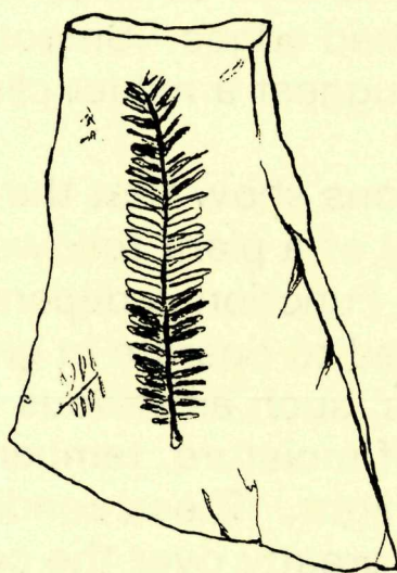
Metasequoia (Dawn Redwood) in shale
