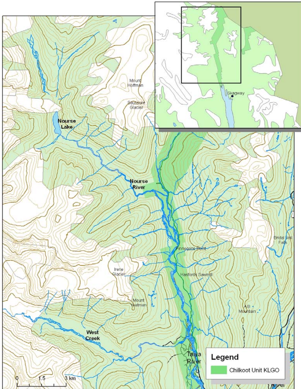
Figure 23. Location of West Creek, Nourse Lake, and the Nourse River, in the Taiya River Watershed. These tributaries have been the source of previous glacial outburst floods on the Taiya River.
