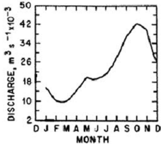
Figure 12. Model-generated values of freshwater discharge in Southeast Alaska based on precipitation, air temperature, and the drainage area of the region, from Royer (1982).
