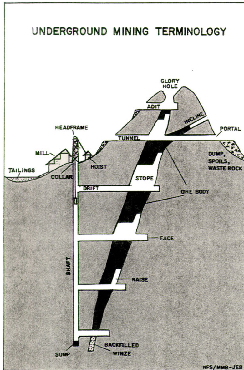
Figure 1. MINING TERMINOLOGY
