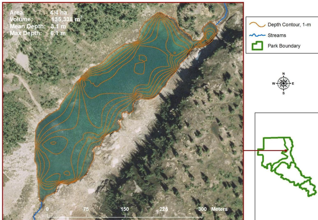
Skymo Lake (PM-03-01) Bathymetry, North Cascades National Park, Aug. 25, 2010
