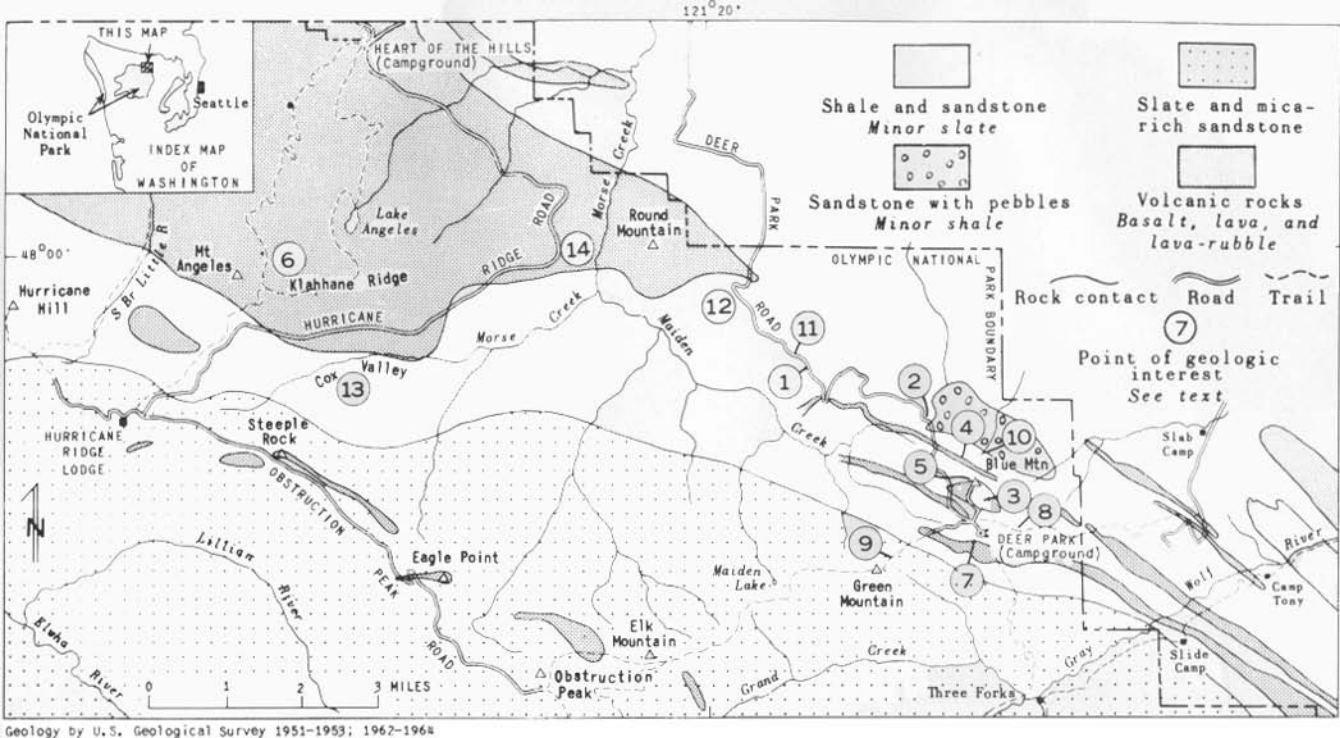
fig. 1. Simplified geologic map of the Mount Angeles - Deer Park area.
