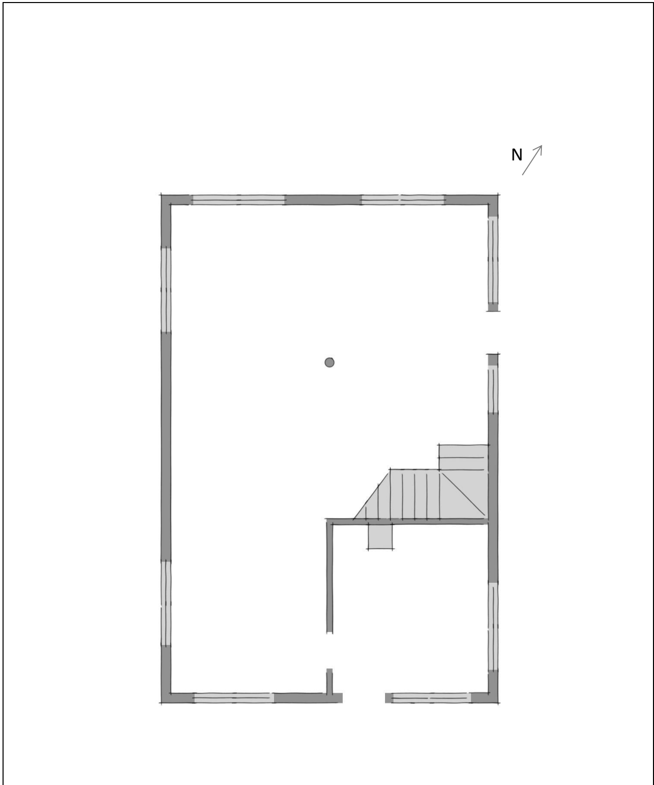
ENCHANTED VALLEY CHALET PLAN—First Floor c. 1930 Historic American Building Survey by Charlotte Helmer Date: August 2014 Scale: 1/8" = 1'-0"
