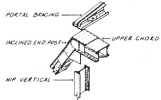
RIVETED CONNECTION
