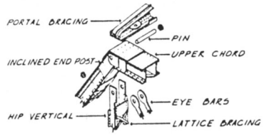
PINNED CONNECTION
