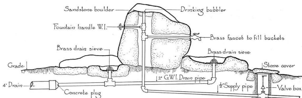
SECTION Scale \frac{3}{8} " = 1'-0"
