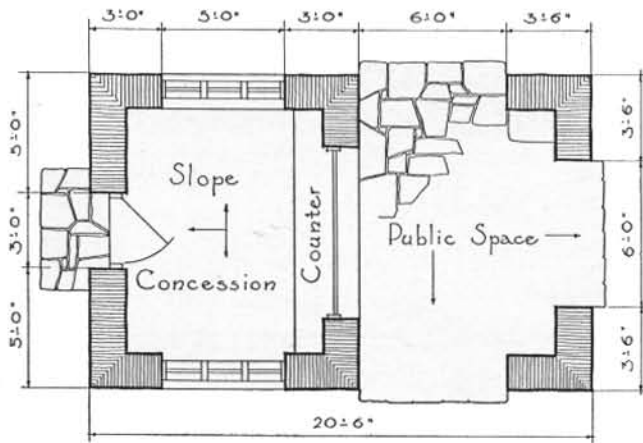
FLOOR PLAN
