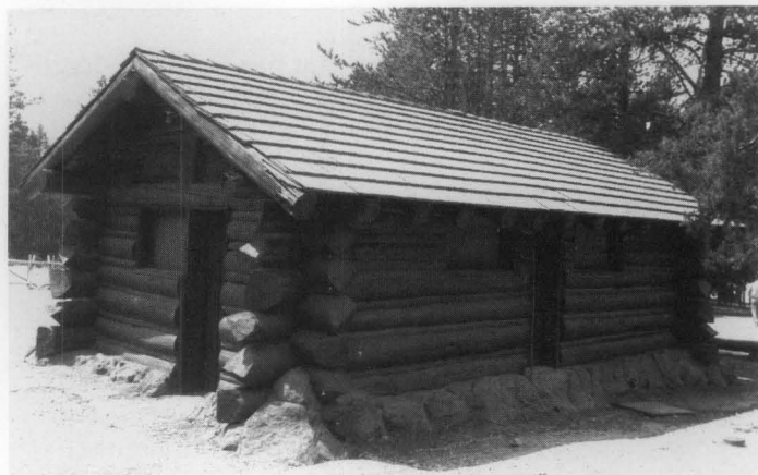
Fig. 18. Exposed roofing members of Rustic style buildings such as this structure at Yellowstone National Park are highly susceptible to deterioration. Photo: Laura Soulliere Harrison.
