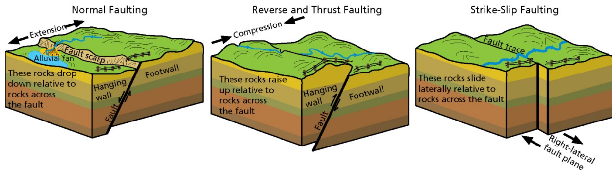
Figure 9. Schematic illustrations of fault types. Movement occurs along a fault plane. Footwalls are below the fault plane and hanging walls are above. In a normal fault, crustal extension (pulling apart) moves the hanging wall down relative to the footwall. In a reverse fault, crustal compression moves the hanging wall up relative to the footwall. A thrust fault is similar to a reverse fault, but has a dip angle of less than 45°. In a strike-slip fault, the relative direction of movement of the opposing plate is lateral. When movement across the fault is to the right, it is a right-lateral (dextral) fault, as illustrated above. When movement is to the left, it is a left-lateral (sinistral) fault. A strike-slip fault between two plate boundaries is called a transform fault. Graphic by Trista Thornberry-Ehrlich (Colorado State University).
