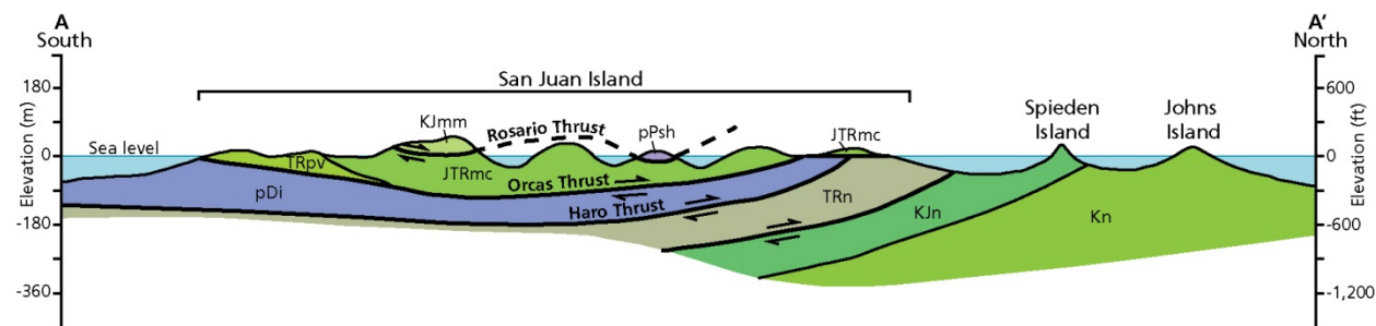
Figure 10. South-north geologic cross section (A-A') showing the subsurface structure of San Juan Island. The cross section suggests that the following deformation events occurred: (1) a thrust transported older Triassic rocks of the Haro Formation (TRn) over Jurassic and Cretaceous units (KJn, Kn), (2) the Haro Thrust transported the pre-Devonian Turtleback Complex (pDi) over the Haro Formation, (3) the Orcas Thrust juxtaposed the Deadman Bay terrane (TRpv, JTRmc) above the Turtleback Complex, (4) the Rosario Thrust transported the Constitution Formation (KJmm) over the Deadman Bay terrane, and (5) the sequence was then folded into a broad syncline. Graphic redrafted by Trista Thornberry-Ehrlich (Colorado State University) after Logan (2003).
