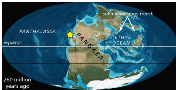
Figure 26. Pangaea. During the Permian and Early Triassic, North America became part of the supercontinent Pangaea. This C-shaped landmass stretched from pole to pole and surrounded the Tethys Ocean. The spine of the "C" was adjacent to a long subduction zone. Much of Earth's surface was covered by a large ocean called Panthalassa. The terranes that accreted to present-day Washington (yellow star) during the Mesozoic originated some distance from the western margin, and the Deadman Bay terrane originated in the Tethys Ocean. Base paleogeographic image by Ron Blakey (Colorado Plateau Geosystems, Inc.), available at http://cpgeosystems.com/index.html (accessed 25 January 2012). Annotations by Jason Kenworthy (NPS Geologic Resources Division).
