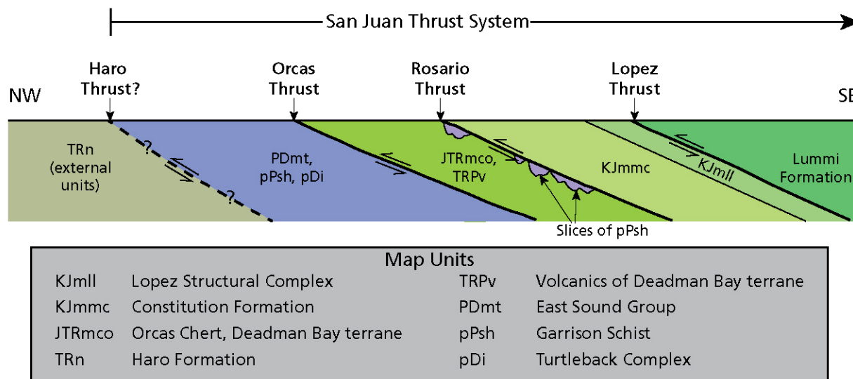
Figure 11. Schematic cross section of the San Juan Thrust System. The Rosario Thrust, which is the dominant thrust on San Juan Island and in San Juan Island National Historical Park, separates the Paleozoic and lower Mesozoic units in the lower part of the San Juan Thrust System from the younger, upper Mesozoic units in the upper part of the system. Arrows indicate direction of movement. Diagram modified from Brandon et al. (1988, fig. 4) by Trista Thornberry-Ehrlich (Colorado State University).
