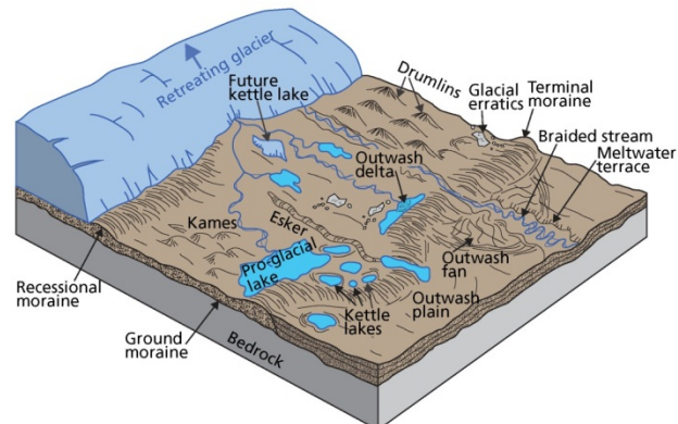
Figure 14. Schematic illustration of various alpine and continental glacial features. Not all features on the illustration are found in all glacial landscapes. Glacial features in San Juan Island National Historical Park include moraines, outwash plains, and glacial erratics. Graphic by Trista Thornberry-Ehrlich (Colorado State University).
