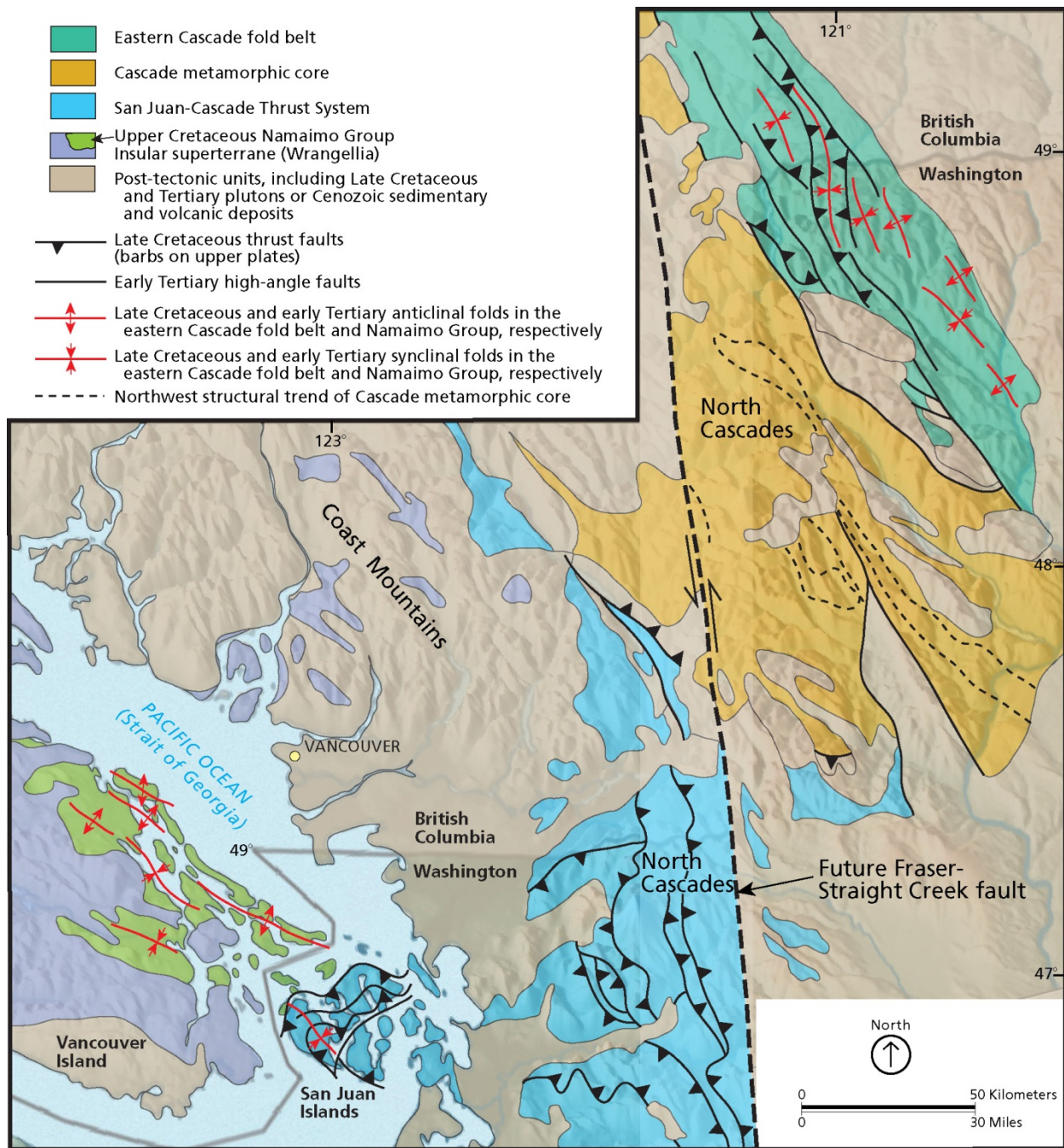
Figure 3. Simplified regional geologic map. This map shows modern geographic features and the four major tectonic terranes that accreted to Washington's western margin during the Cretaceous: (1) Wrangellia, (2) San Juan-Cascade Thrust System (San Juan Thrust System), (3) Cascade metamorphic core, and (4) eastern Cascade fold belt. Wrangellia, a large terrane that is part of the larger Insular Superterrane, lies west of the San Juan Archipelago and composes most of Vancouver Island. The northwest-southeast-trending San Juan Thrust System includes the San Juan Islands and the Cascade Mountains of northwestern Washington. The other two tectonic zones lie east of the San Juan Thrust System. Graphic by Trista Thornberry-Ehrlich (Colorado State University), redrafted after Cowan and Brandon (1994, fig. 2) using basemap by Tom Patterson ( http://www.shadedrelief.com/physical/pages/download.html ; accessed 4 April 2014).
