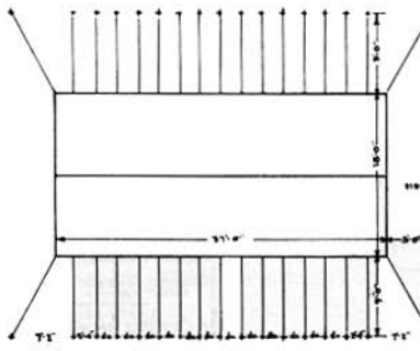
PLAN OF STAKING FOR 18x37 WALL TENTS SCALE: 1/8"=1'-0"
