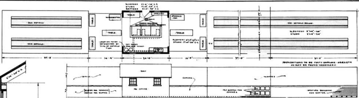
SIDE ELEVATION OF KITCHEN & MESS UNITS SCALE: 1/8"=1'-0"
