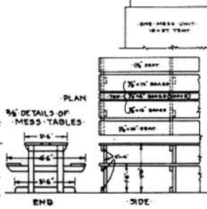
3/4" DETAILS OF MESS TABLES END SIDE
