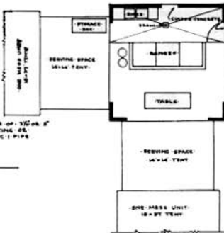
ALTERNATE PLAN SHOWING THREE MESS WINGS SCALE: 1/8"=1'-0"
