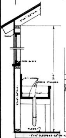
3/4" SCALE KITCHEN DETAILS
