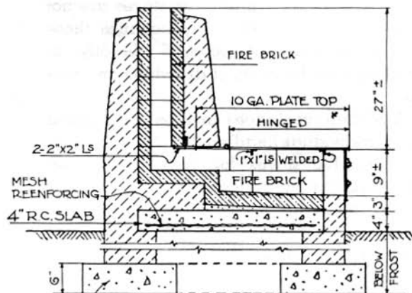
SECTION "C-C" FIG. 4
