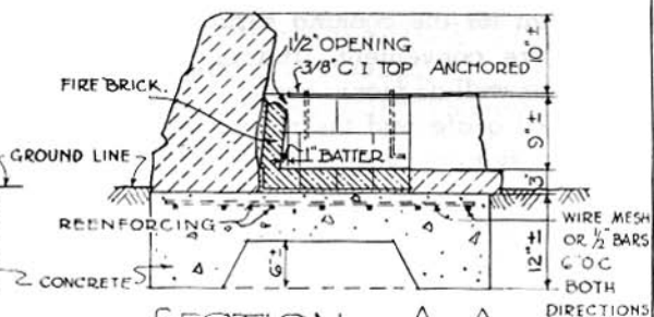
SECTION A-A FIG 3
