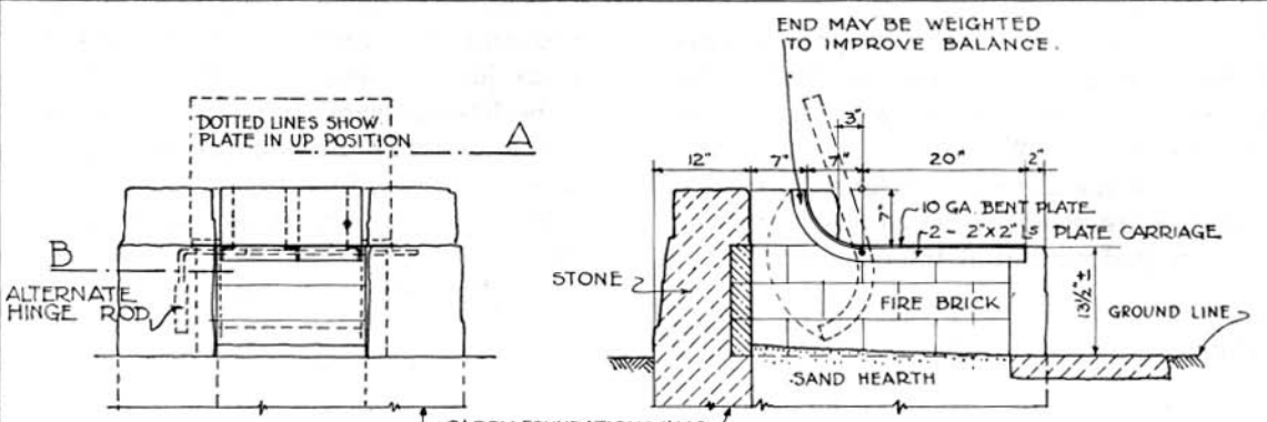
ELEVATION FIG 3
