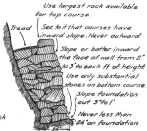
Showing cross section of a correctly laid rock wall.
