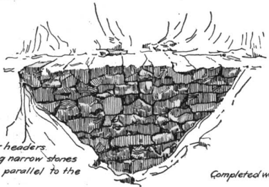
Showing cross section of a correctly laid rock wall.
