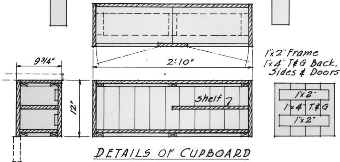
LASSEN TABLE WITH CUPBOARDS SCALE 1" = 1'-0"
